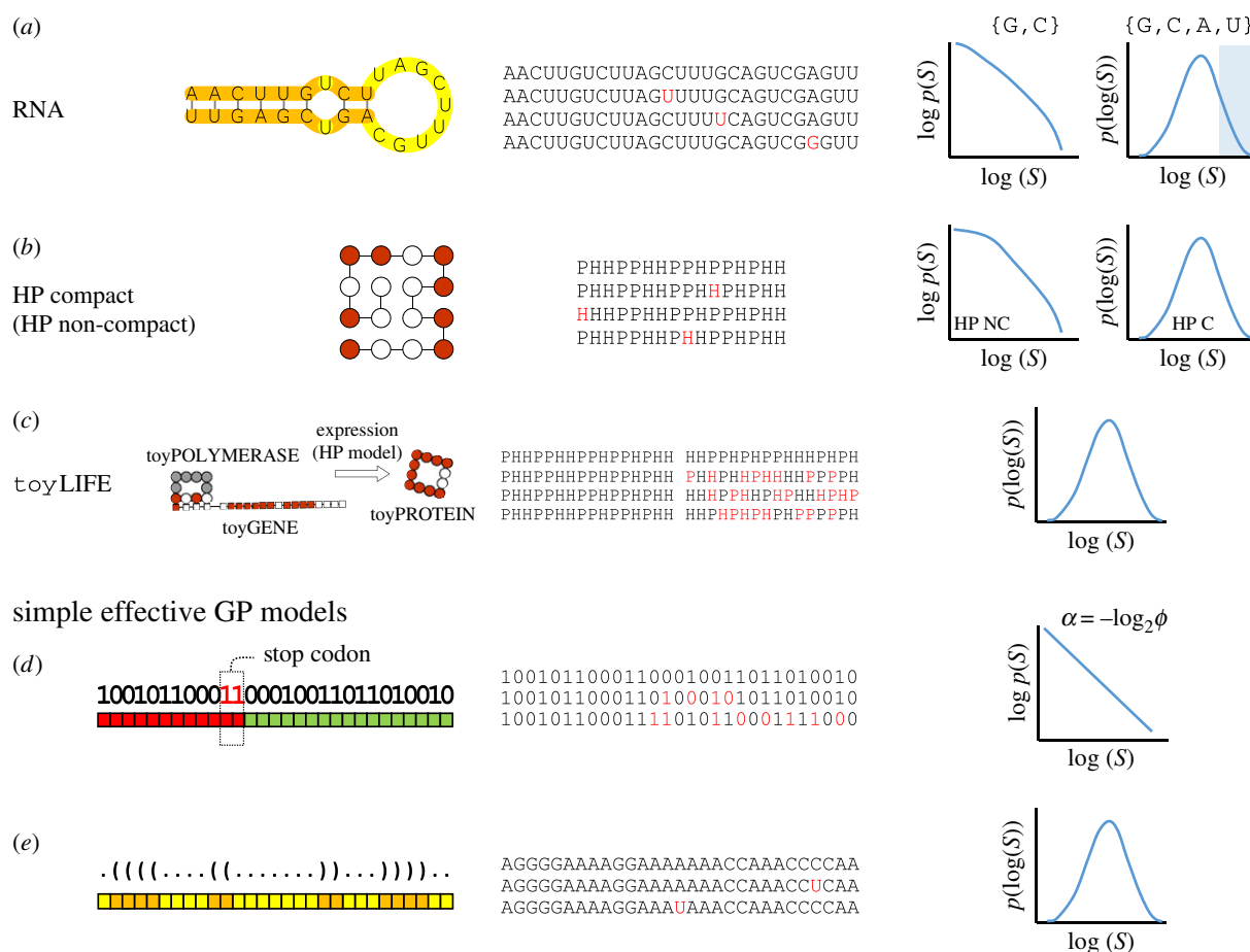
Figure 2. Some examples of simple GP maps. For each model, and from left to right, we depict an example phenotype, some of the sequences in its neutral network (mutations that do not change the phenotype are highlighted in red), and the schematic functional form of the probability distribution p(S) of phenotypes sizes S found in computational or analytical studies. (a) RNA sequence-to-minimum-free-energy secondary structure. Mutations that do not disrupt the secondary structure appear with different probability in loops or stacks. In two-letter alphabets, the distribution of phenotype sizes is compatible with a power-law function [49], while in four-letter alphabets p(S) is well fit by a lognormal distribution [50]. For long sequences, only the right-most part of p(S) can be seen under random sampling of the genotype space [50] (shaded). (b) The HP model, in its compact (as in the figure) or non-compact versions, has been studied as a model for protein folding. In non-compact versions, the distribution p(S) has a maximum at S = 1 and decays with a fat tail [51], while in compact versions p(S) resembles a lognormal distribution [52]. (c) \text{toyLIFE} is a minimal model with several levels. HP-like sequences are read and translated to proteins that interact through analogous rules to break metabolites. The p(S) of \text{toyLIFE} is compatible with a lognormal distribution [53]. (d,e) Effective models where phenotype is defined in relation to the composition of sequences allow to analytically calculate the functional form of p(S) . Two examples are (d) Fibonacci's model [54], where p(S) follows a power-law distribution and (e) an RNA-inspired model [55] which yields a lognormal distribution of p(S) .
