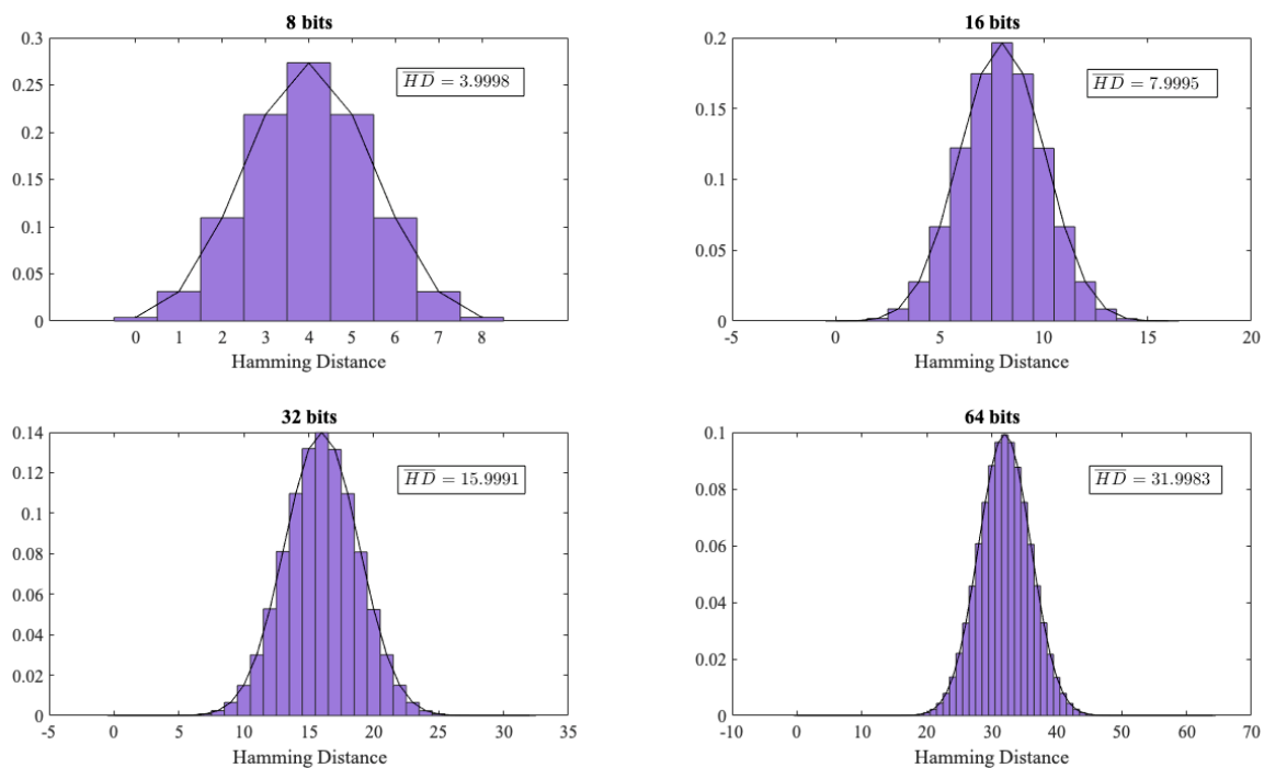
Figure 5. Hamming distance distribution.
