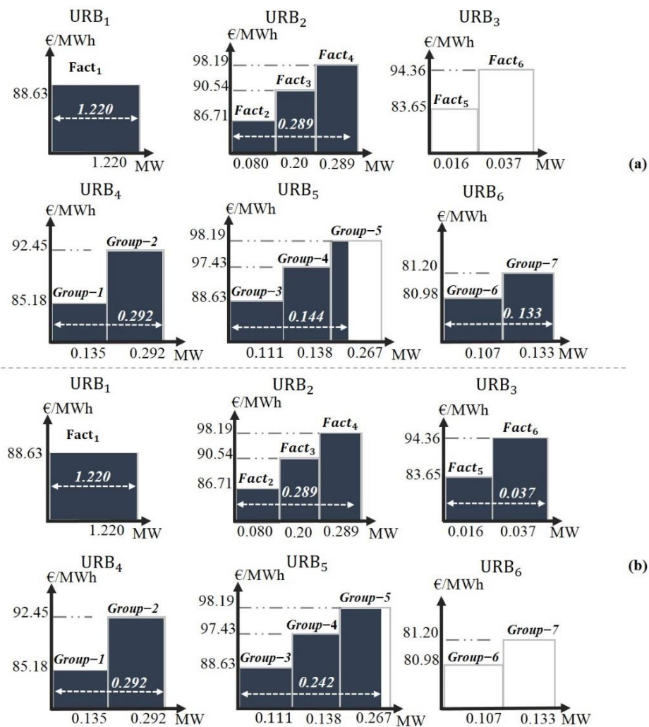
Figure 8. Two possible feasible combinations of bids (a) and (b), resulting from stage 1 of optimization at hour 19.
