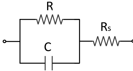
Figure 3. Equivalent electric circuit of a LC cell for a frequency range of 100 to 10^5 Hz.
