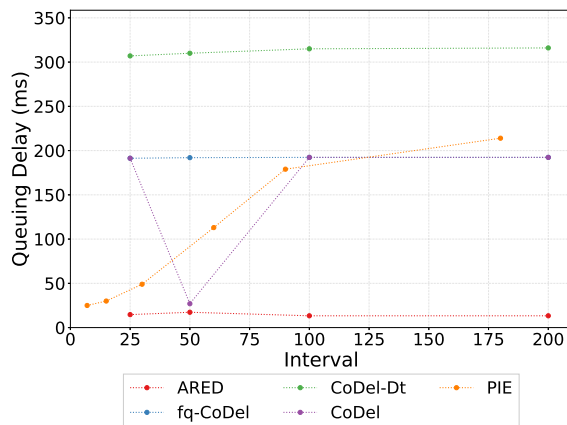
Figure 6.11: Lebat: Delay vs. Interval
