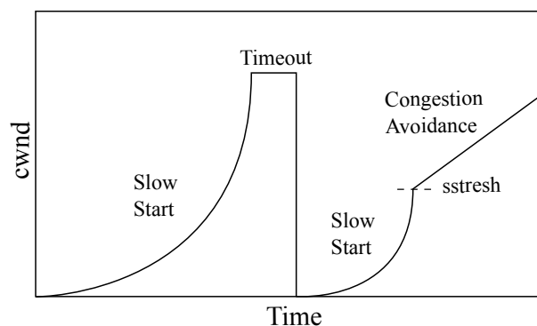
Figure 2.1: New Reno cwnd evolution
