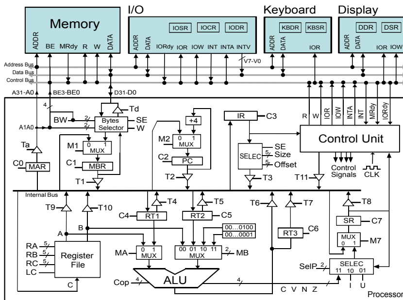
Figura A-1: CPU Architecture WepSIM.
