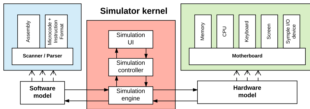
Figura A-3: WepSIM Architecture .
