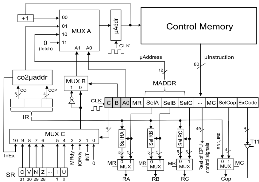
Figura A-2: Control unit architecture in WepSIM.
