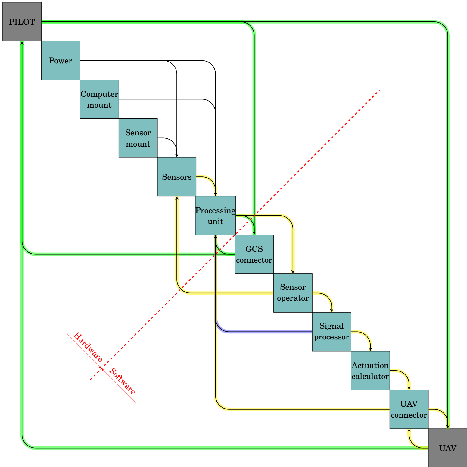
Figure 5.13: OCAS N 2 diagram for interfaces definition
