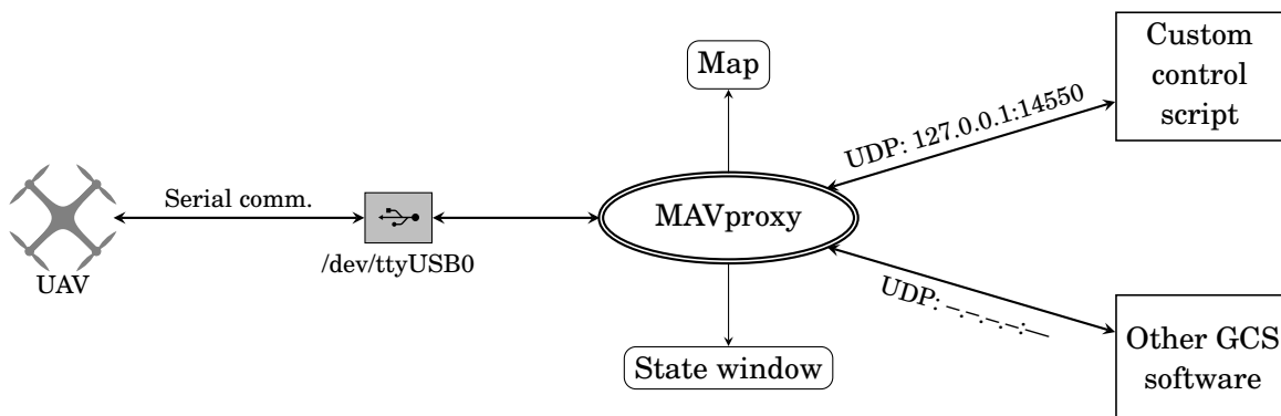
Figure 6.11: MAVproxy setup
