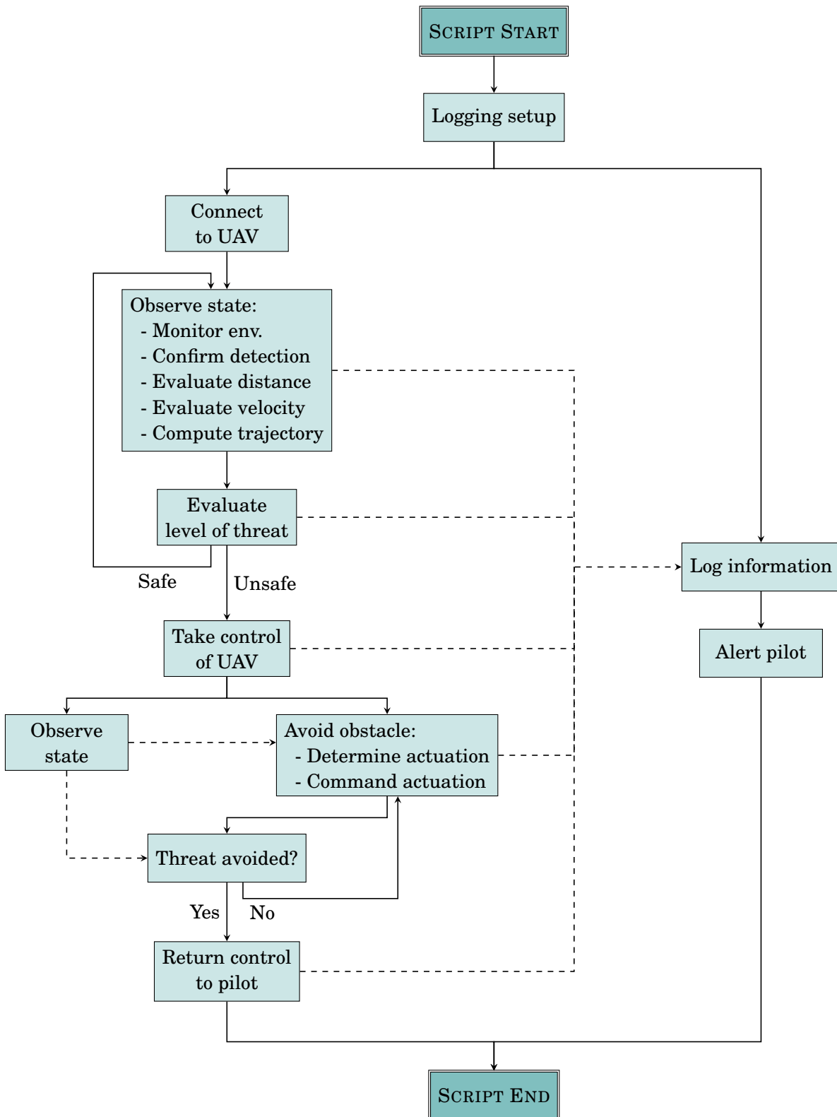
Figure 6.12: Functional flow diagram of the Python script
