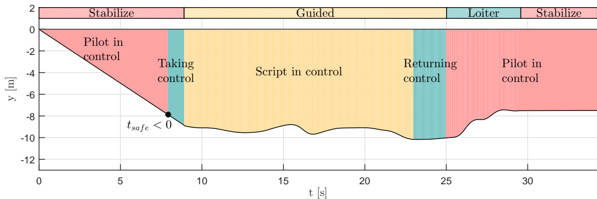
(b) Longitudinal position during the flight test
