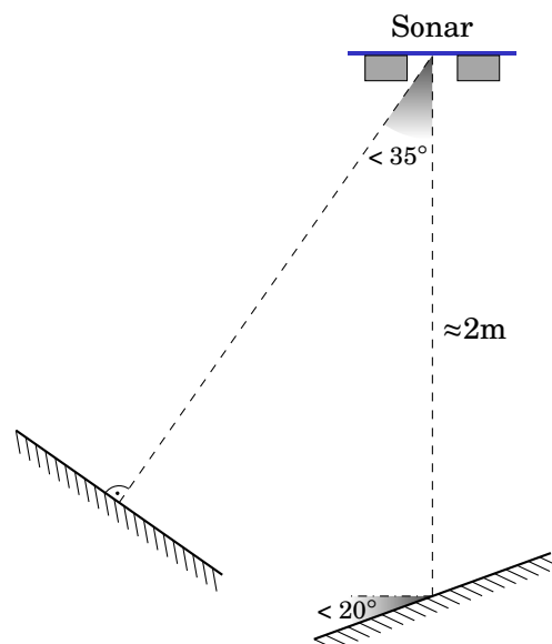
Figure 7.2: Ultrasonic rangefinder FOV test setup
