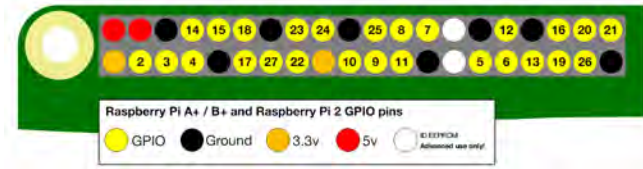
Figure 6.7: GPIO pins on the Raspberry Pi 2 model B Source: raspberrypi.org
