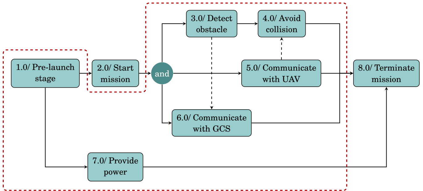
Figure 5.5: OCAS Functional Flow Block Diagram. TOP LEVEL
