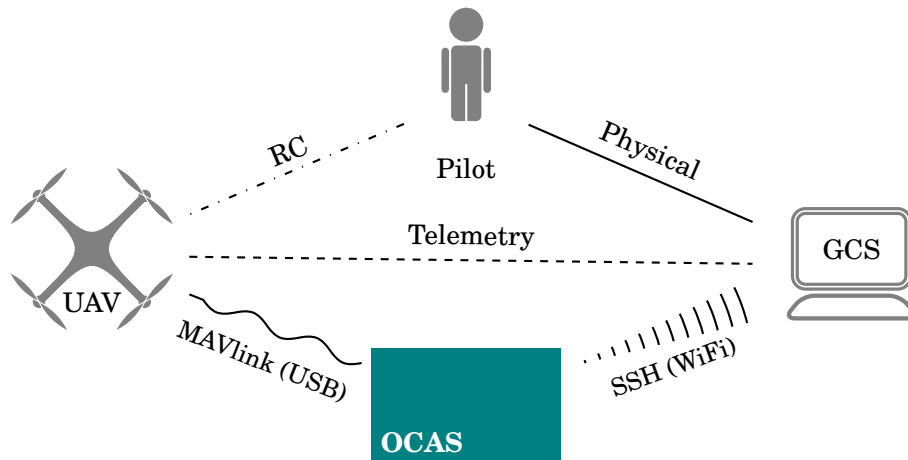
Figure 6.2: OCAS-equipped UAS architecture
