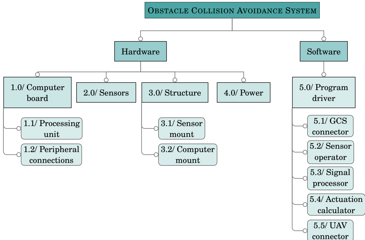
Figure 5.11: OCAS Product Breakdown Structure
