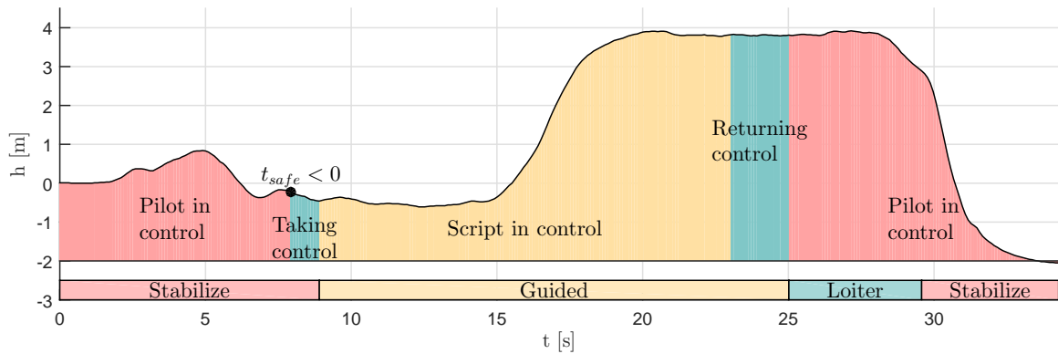
(a) Relative altitude during the flight test
