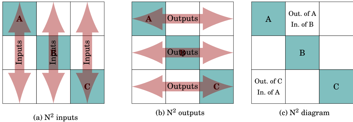
Figure 5.12: Example of a N^2 diagram
