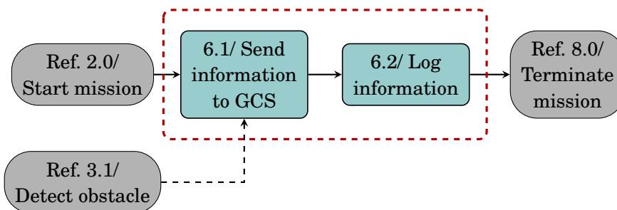
Figure 5.10: OCAS Functional Flow Block Diagram. 6 th STAGE
