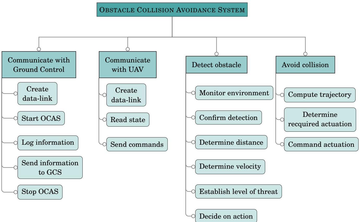
Figure 5.3: OCAS Functional Architecture
