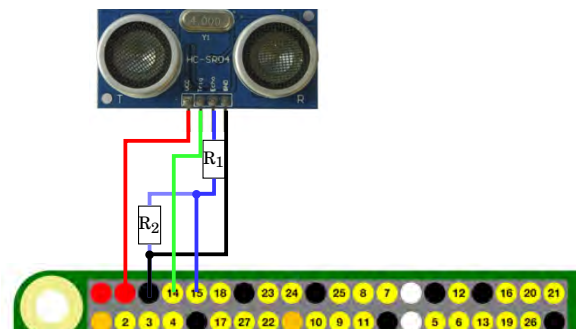
Figure 6.9: Connection of the HC-SR04 sensor to the Raspberry Pi
