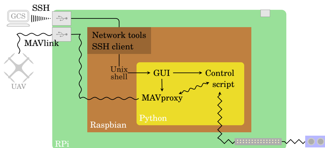
Figure 6.10: Software architecture of the OCAS computer
