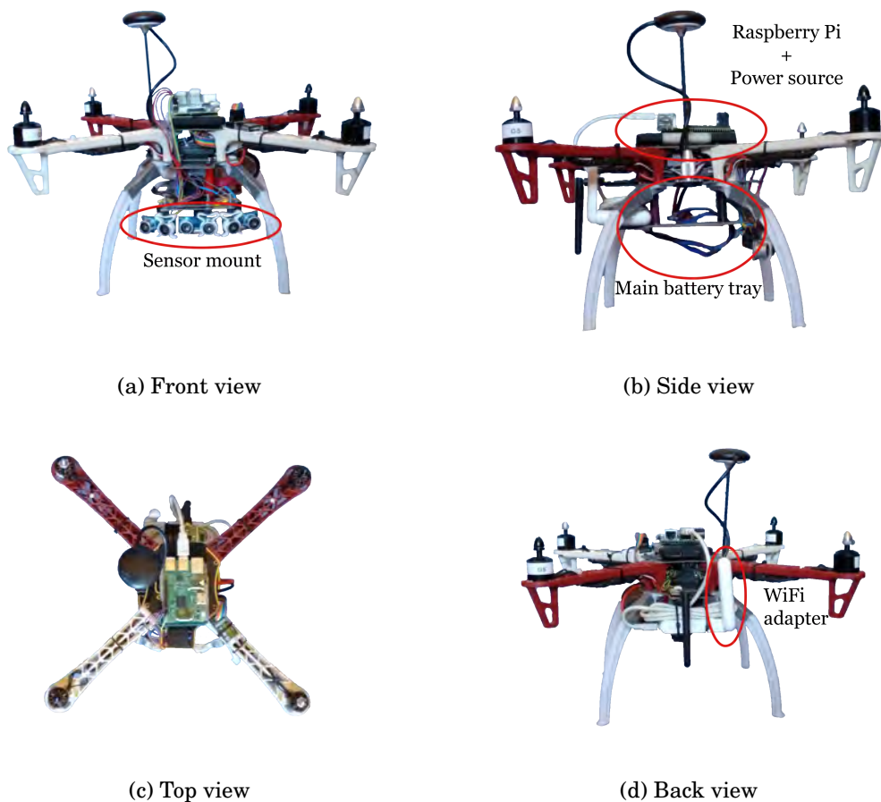
Figure 6.16: Final platform architecture
