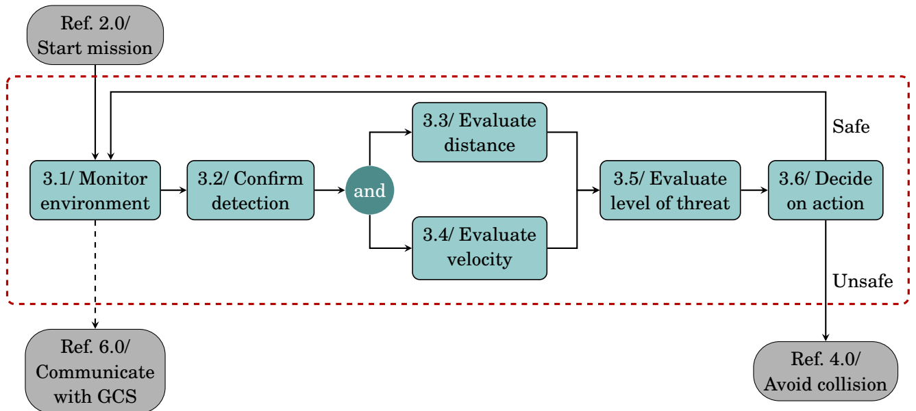
Figure 5.7: OCAS Functional Flow Block Diagram. 3 rd STAGE
