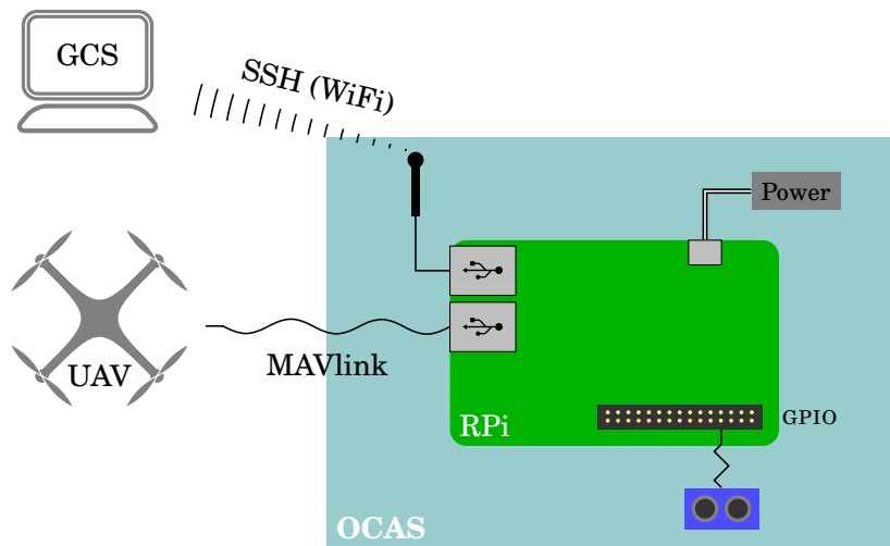
Figure 6.6: OCAS hardware layout
