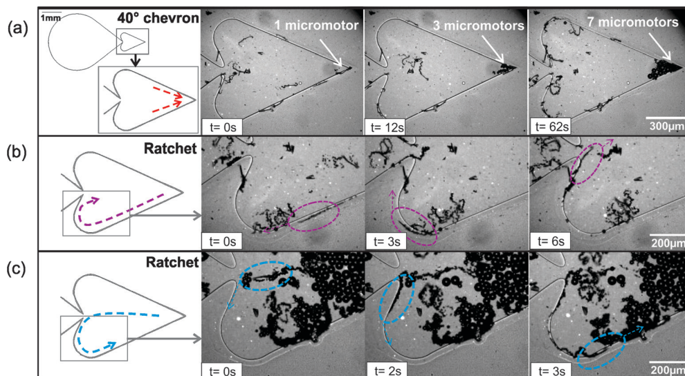
Fig. 3 Trapping mechanisms in the heart-shaped structure. Left panels show the design of the heart-shaped reservoir (a) time lapse images of micromotors being trapped in the 40^\circ chevron. A total of 7 micromotors are trapped in ca. 1 min (b) Micromotors swimming towards the center and (c) from the center along the walls of the ratchet mechanism are retained in the trapping chamber. The red, pink and blue arrows on the schematics of the left-side figures indicate the trajectories of the micromotors.
