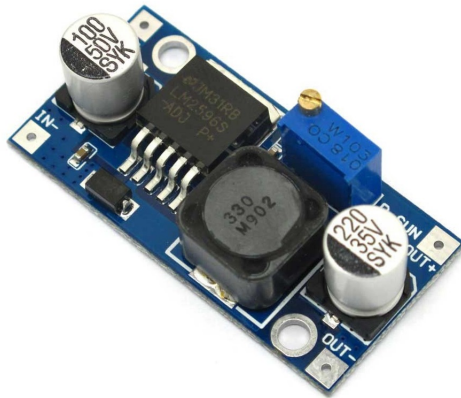
Figure 10: LM2596S step-down converter
