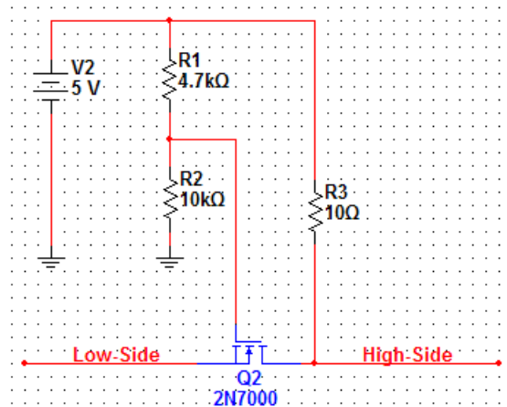
Figure 11: Bidirectional voltage converter
