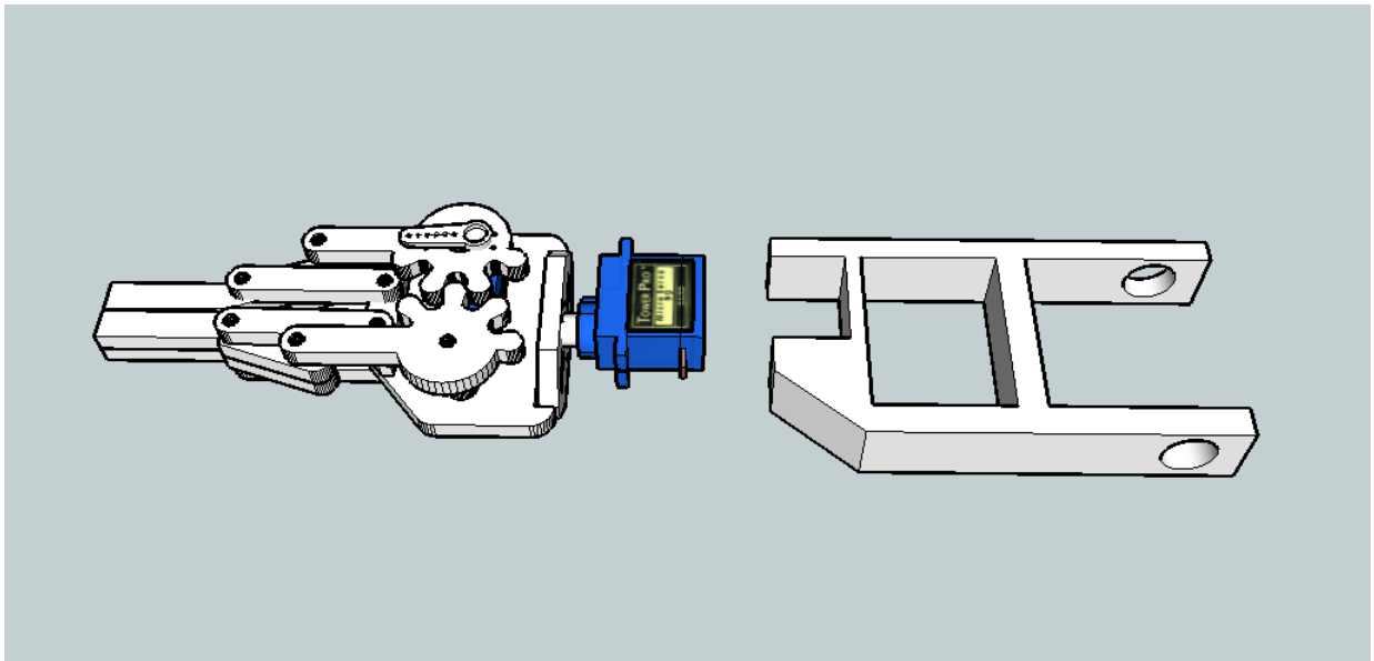
Figure 27: Connection of the gripper to the forearm
