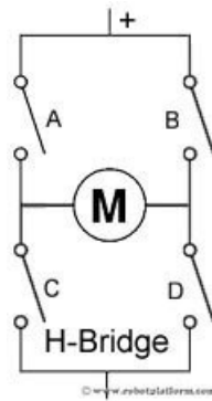
Figure 14: H-bridge circuit
