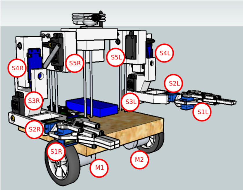
Figure 46: Detail of the robot’s actuators
