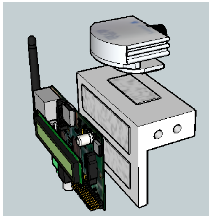
Figure 38: Coupling of the electronics to the robot's head
