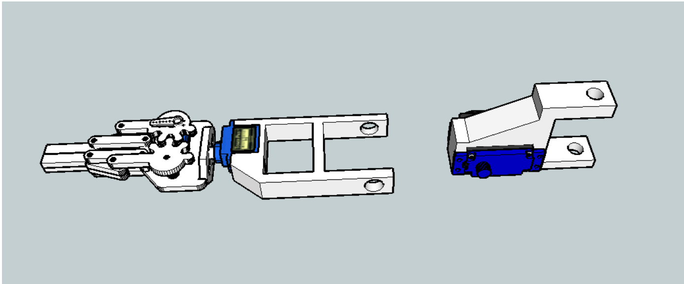
Figure 29: Linkage of the elbow to the forearm
