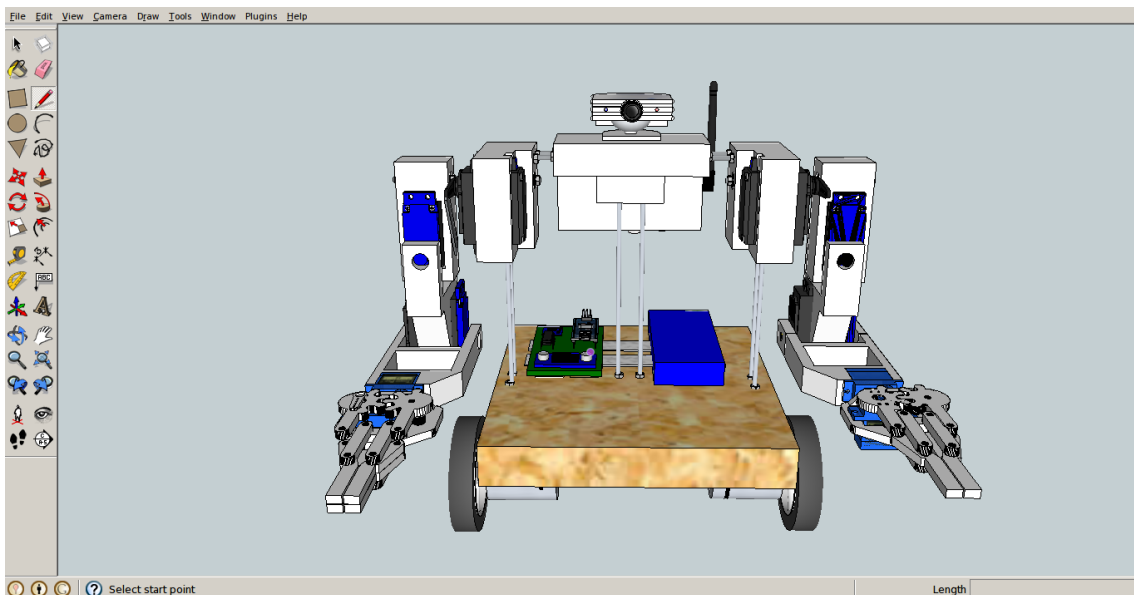
Figure 7: SketchUp software
