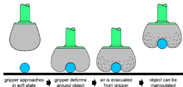
Figure 60: Vacuum gripper
