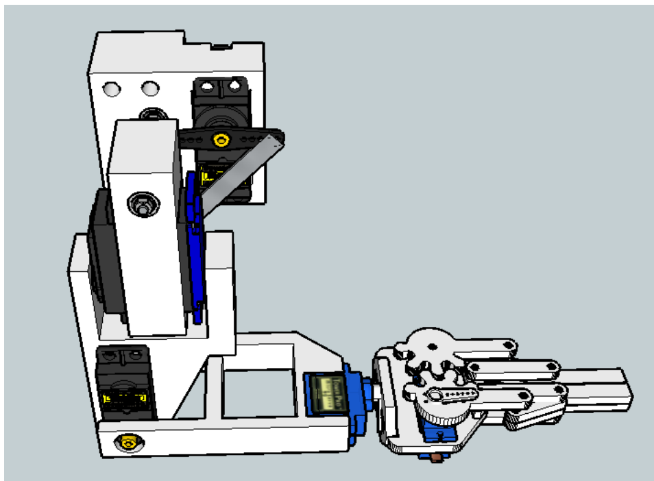
Figure 35: Detail of linkage between the shoulder servo and the upper arm
