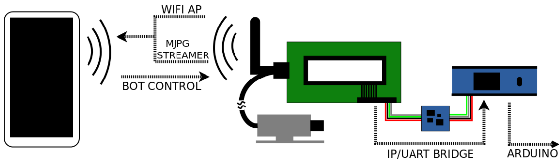
Figure 52: Software connections diagram
