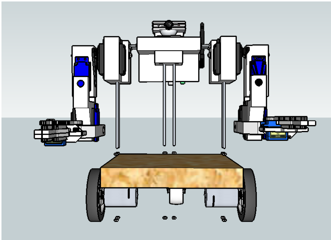
Figure 42: Connection of upper body to base
