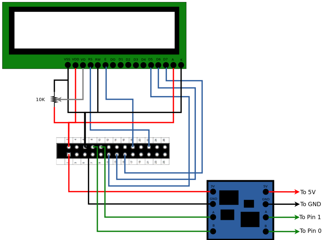
Figure 48: Detail of LCD and Serial connections
