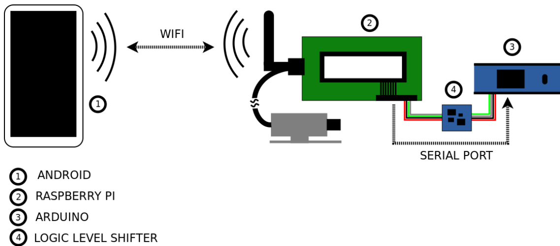
Figure 51: Logic connections diagram
