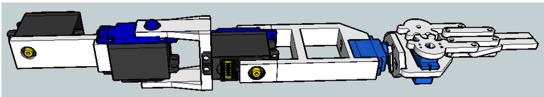
Figure 23: Initial arm design
