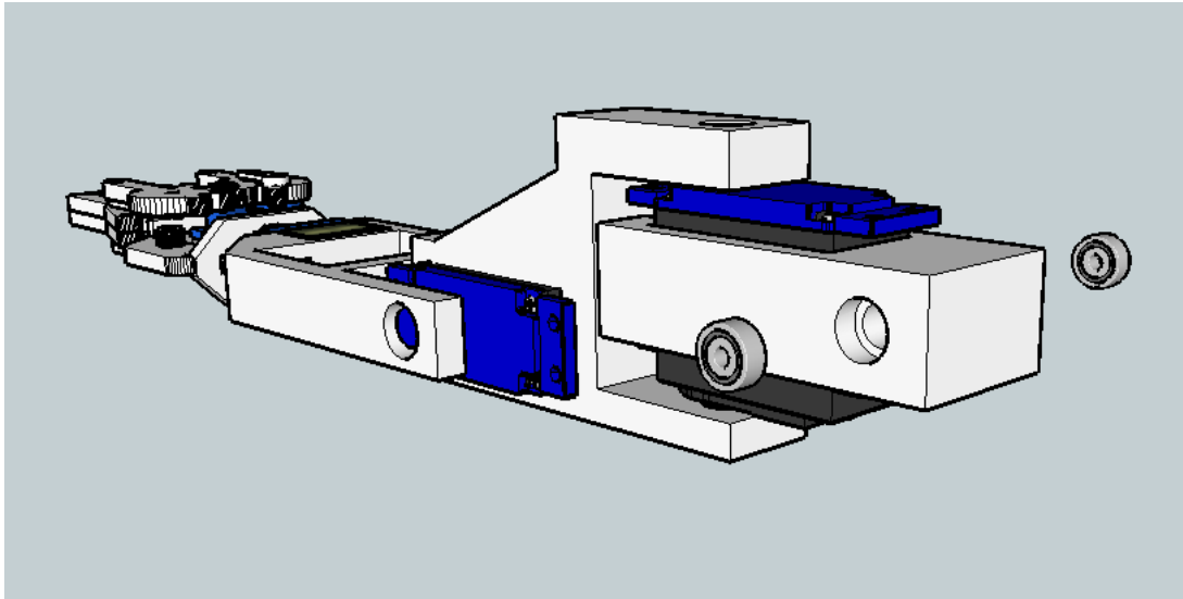
Figure 32: Detail of bearings insertion into the upper arm
