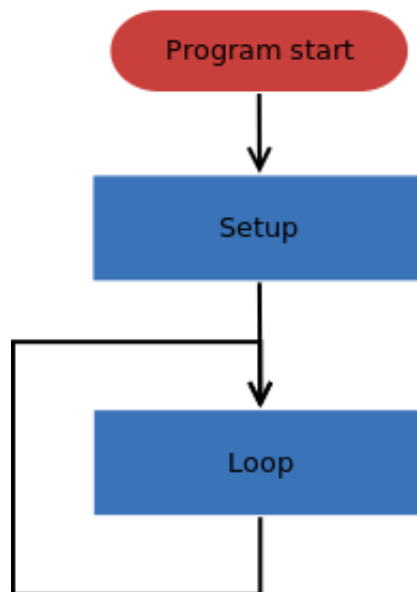
Figure 53: Arduino code skeleton
