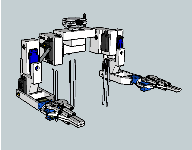
Figure 40: Detail of support rods insertion
