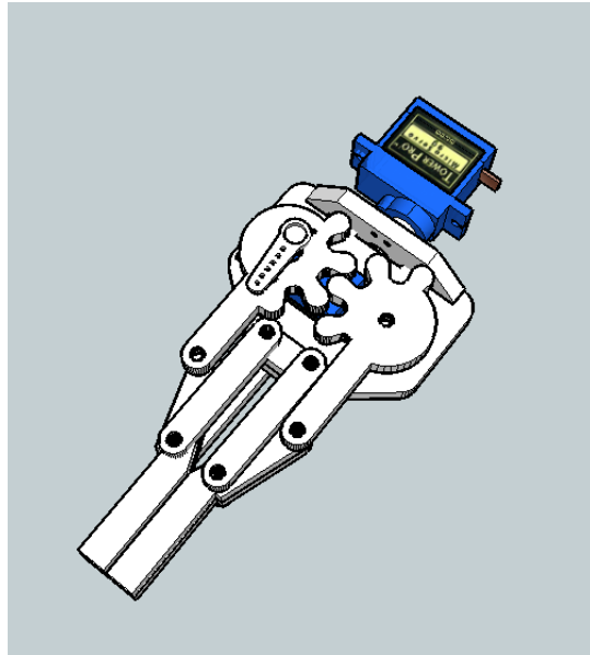
Figure 26: Detail of the gripper assembled
