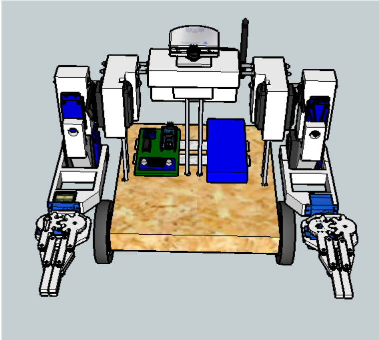
Figure 45: Assembled robot
