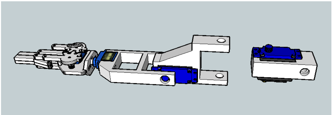
Figure 31: Coupling of the upper arm to the elbow
