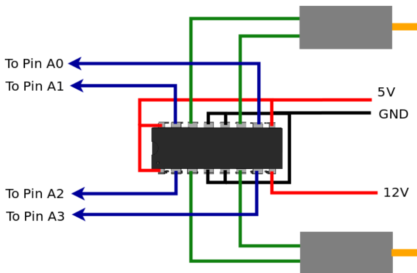
Figure 49: Detail of motor driver wiring
