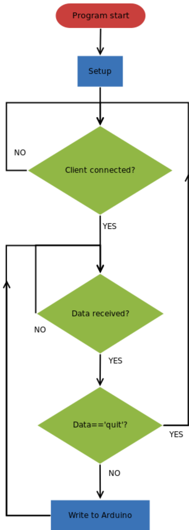
Figure 56: IP/UART program flowchart
