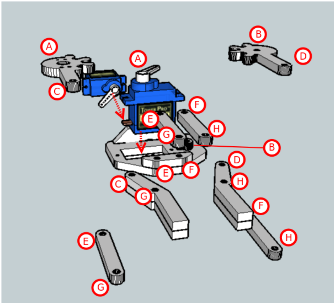
Figure 25: Assembly of the gripper
