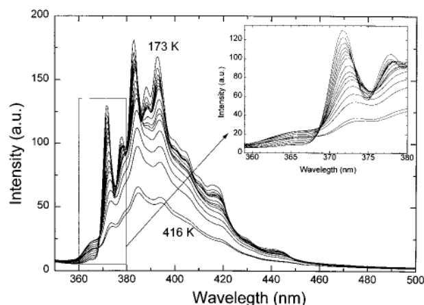
Figure 2. Fluorescence emission spectra of pyrene in low-density polyethylene at several temperatures, obtained during a heating cycle at a rate of 2 \text{ }^\circ\text{C}/\text{min} . The insert expands the wavelength region in which an isoemissive point is observed.
