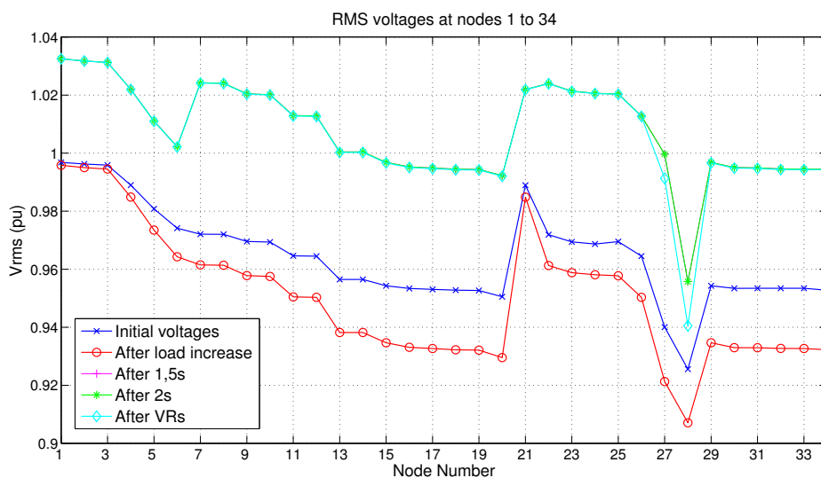
(a) Time delay increases downstream
