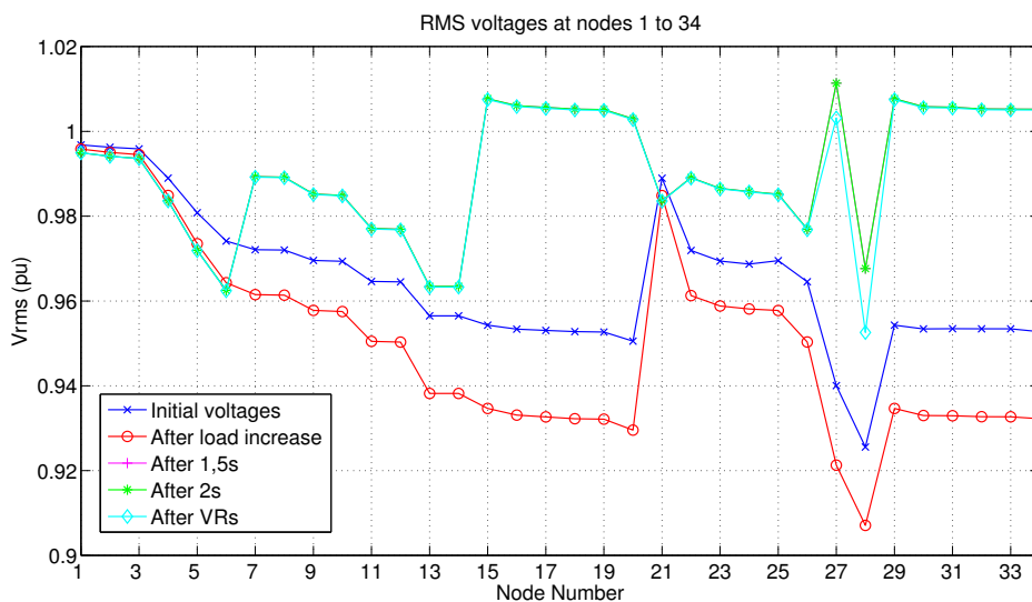
(b) Time delay decreases downstream
