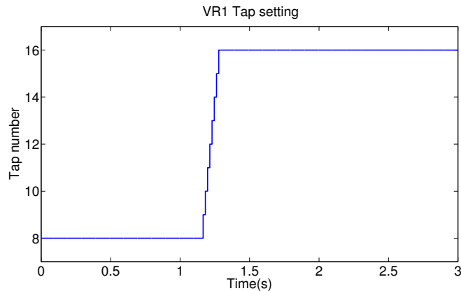
(b) Tap changes at Voltage regulator
