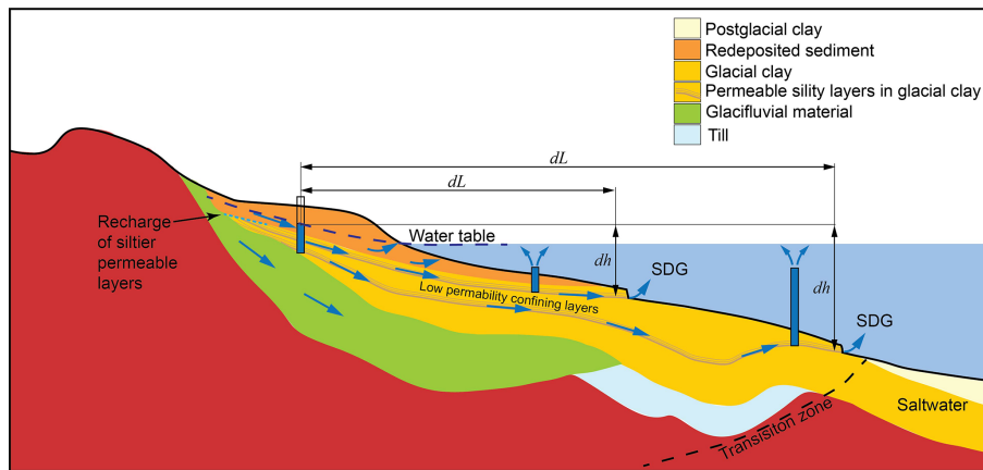
Figure 9. Schematic illustration showing how siltier layers in glacial clay could act as a conduit for groundwater, eventually escaping at the sea floor as SGD and leading to the formation of a bathymetric terrace. The critical parameters dh and dL in Darcy's law (Eq. 2) are illustrated in the sketch as they dictate the hydraulic head that would drive the flow.
