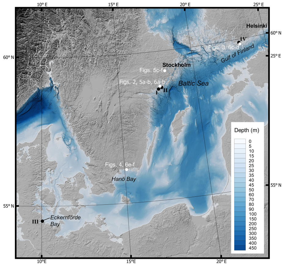
Figure 1. Overview map showing the locations of the studied areas in this work with white dots. Corresponding figures for each area are shown with white text. The locations of previous studies showing SGD discussed here are shown with black dots. I and II: Söderberg and Flodén (1997); III: Schlüter et al. (2004); IV: Virtasalo et al. (2019). The bathymetry is from EMODnet 2018 (EMODnet Bathymetry Consortium, 2018)
