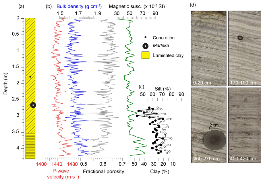
Figure 7. Lithology and sedimentology of sediment core Asko2018HT-2GC. Image includes a lithologic log (a), sediment physical properties measured on the MSC/L (b), and results from grain size analyses showing variations in clay and silt content across the zone where the overall porosity reduction is seen ( \sim 3.5 m) (c). Characteristic images from four different depths are shown (d), including the 2 cm diameter concretion recovered at 2.64 m and the smaller concretion at 1.77 m.
