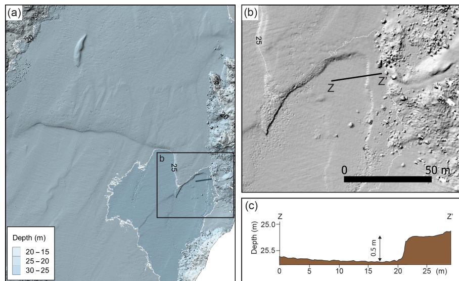
Figure 4. Multibeam bathymetry of a terrace mapped in the southern Blekinge archipelago. (a) Only a smaller part of the full survey is shown without coordinates because detailed bathymetric information from this area is under military restrictions. (b) Detail of the > 500 m long terrace with the location of the bathymetric profile from Z - Z' shown in (c) .
