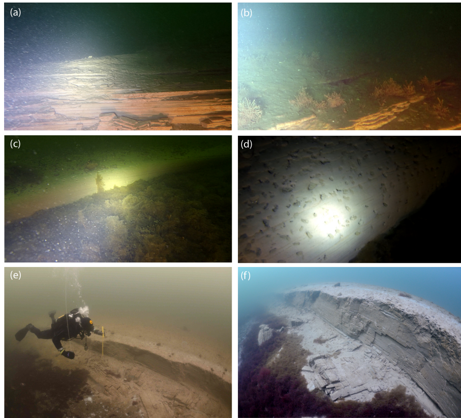
Figure 6. Bottom photographs of sea floor terraces in the studied areas. (a, b) East of the island of Askö, (c, d) east of Tvärminne Zoological Station in the southern Finland archipelago, (e, f) near Boön, Blekinge archipelago.
