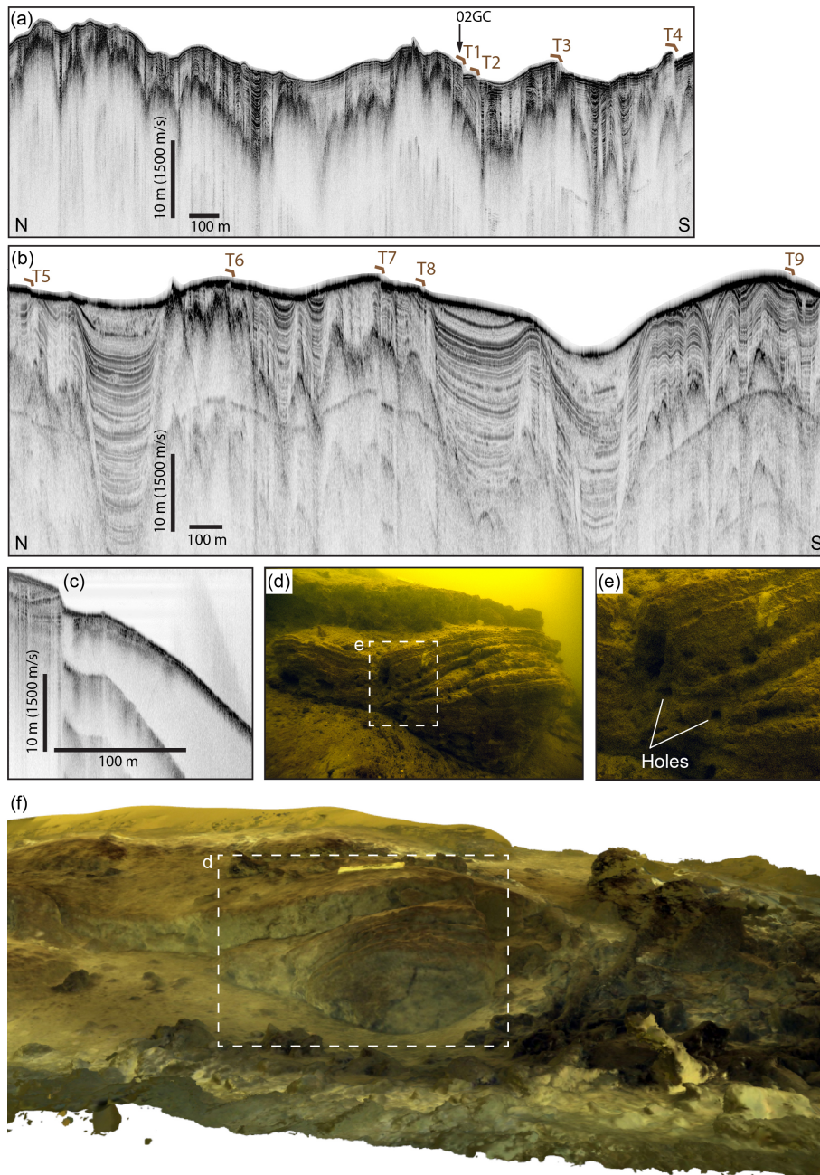
Figure 5. Sub-bottom profiles and bottom photographs portraying sea floor terraces. (a, b) Sub-bottom profiles SBP1 (a) and SBP2 (b) from the area east of Askö. The locations of terraces clearly identified in the multibeam bathymetry are marked T1–T9 (see Fig. 2a). The site of core Asko2018HT-2GC (02GC on profile SBP1) is shown with a black arrow. Note that it is located on top of terrace T1. (c) Sub-bottom profile across the terrace mapped west of the island of Kastellholmen in Stockholm Harbour. Bottom photographs are shown in (d, e) and a 3-D photomosaic of this terrace in (f).
