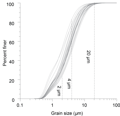
Figure 8. Cumulative grain size distributions for the laminated glacial clays in Asko2018HT-2GC. Sediments are exclusively composed of fine fraction material, with 50%–80% of the sediments being < 4 \mu\text{m} .
