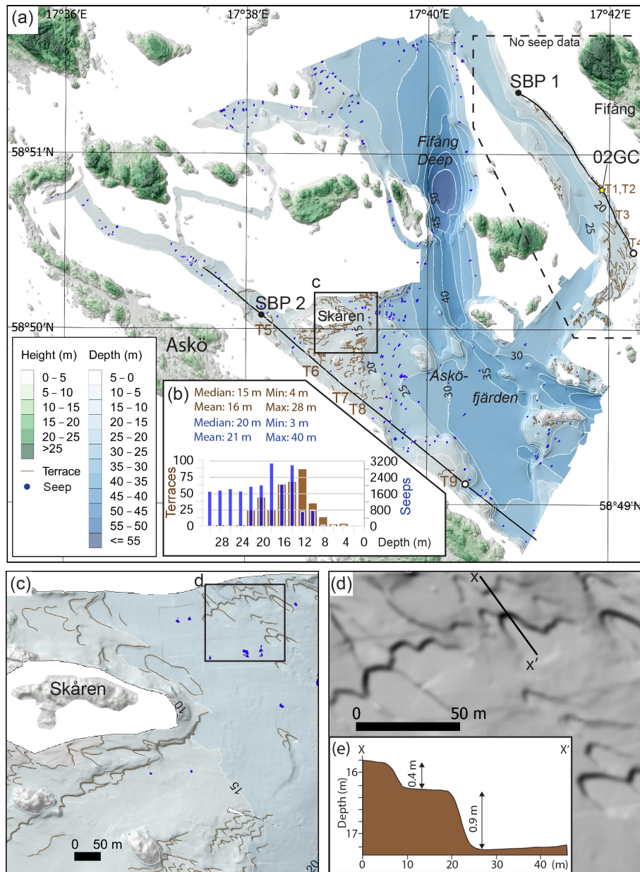
Figure 2. Multibeam bathymetry of the studied area east of the island of Askö, southern Stockholm archipelago. (a) Overview map with brown lines representing digitized terraces in the sea floor and blue dots showing locations where seeps were identified in the multibeam water column data. Black heavier lines show the locations of the sub-bottom profiles in Fig. 5a (SBP1) and b (SBP2). The sub-bottom profiles in Fig. 5 are portrayed between the two dots, with the profile running from left (black dot) to right (white dot). The location of core Asko2018HT-2GC is marked by a yellow star (abbreviation 02GC used on the map). (b) Depth statistics of the occurrence of terraces and seeps. (c) Detailed view of the terraces in the sea floor around the island of Skåren. (d) The location of the bathymetric profile across two terraces from X to X' shown in (e) .
