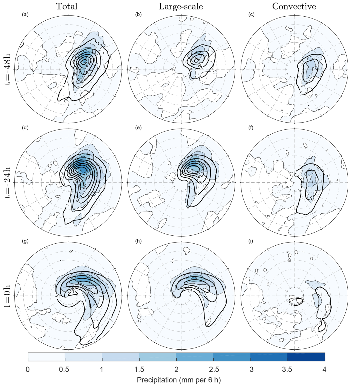
Figure 9. Composites of total precipitation ( a , d , g ), large-scale precipitation ( b , e , h ), and convective precipitation ( c , f , i ) in the CNTL simulation (black contours) and the difference between SST4 and control (shading). Panels ( a )–( c ) are valid 48 h before the time of maximum intensity, panels ( d )–( f ) are valid 24 h before the time of maximum intensity, and panels ( g )–( i ) are valid at the time of maximum intensity. All composites are of the strongest 200 extra-tropical cyclones in each experiment.
