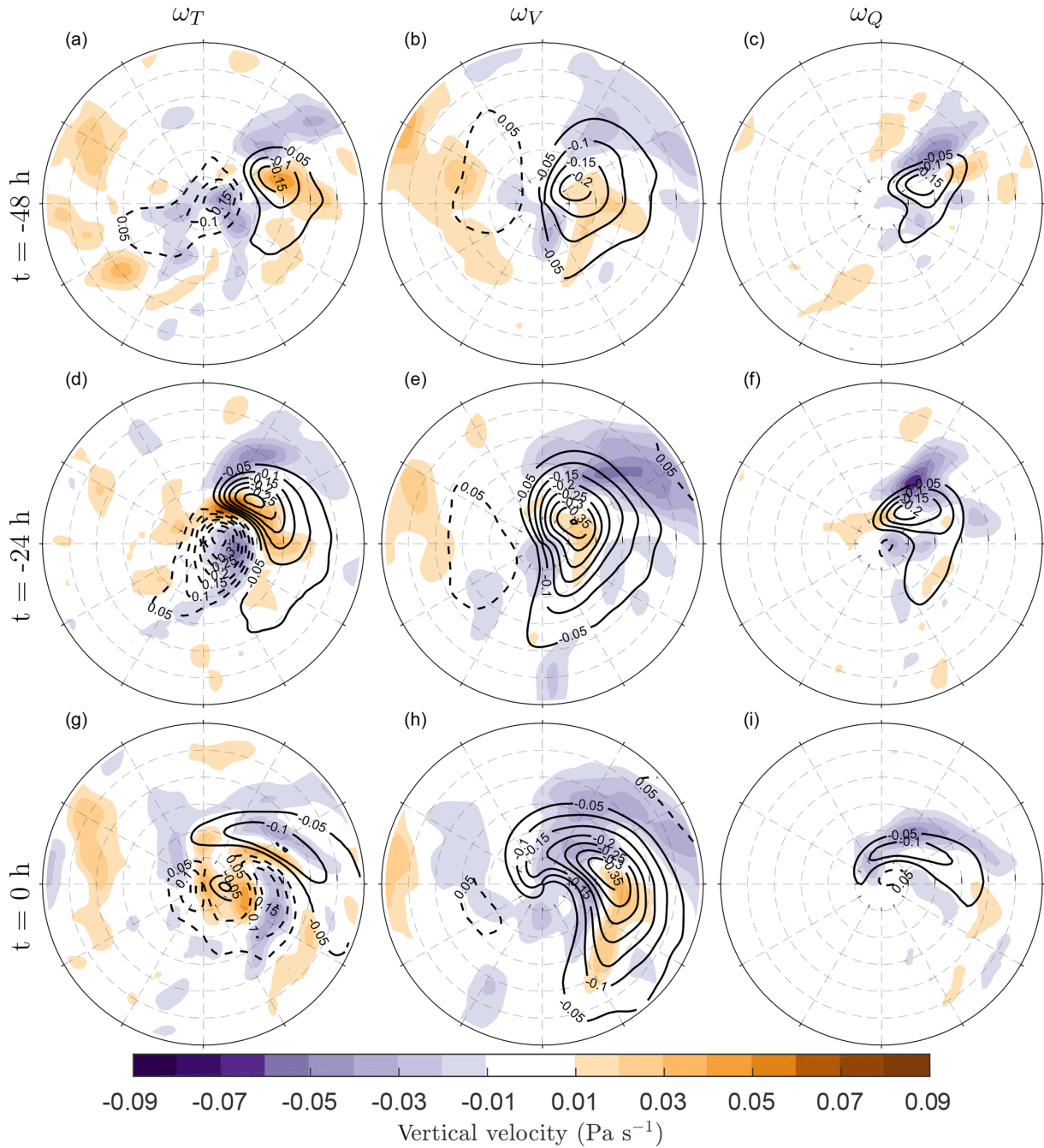
Figure 11. Composite mean and change in 700 hPa vertical velocity in pressure coordinates due to thermal advection ( \omega_T , a, d, g ), due to vorticity advection ( \omega_V , b, e, h ), and due to diabatic heating ( \omega_Q , c, f, i ). Panels (a)–(c) are valid 48 h before the time of maximum intensity, panels (d)–(f) are valid 24 h before the time of maximum intensity, and panels (g)–(i) are valid at the time of maximum intensity. Contours show the control values and shading the difference (SST4 – CNTL). All composites are of the strongest 200 extra-tropical cyclones in each experiment.
