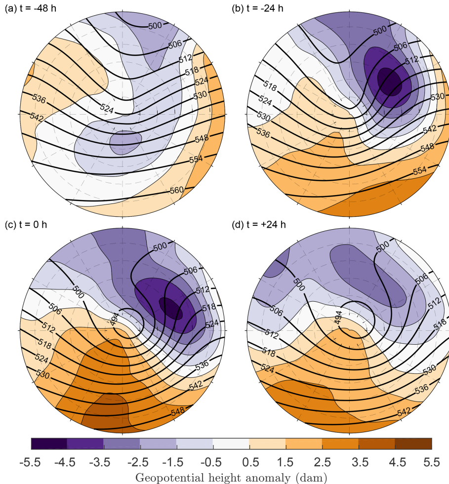
Figure 12. Composite mean of 500 hPa geopotential height (dam) in CNTL (black contours) and the difference (SST4 – CNTL) in the cyclone relative anomalies at (a) 48 h before time of maximum intensity, (b) 24 h before time of maximum intensity, (c) time of maximum intensity, and (d) 24 h after the time of maximum intensity.
