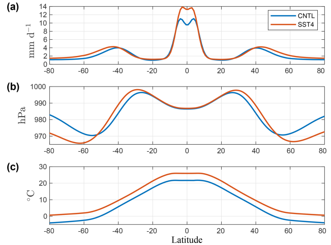
Figure 2. Zonal mean (a) total precipitation (mm d -1 ), (b) mean sea level pressure (hPa), and (c) 950 hPa temperature (°C) averaged over 10 years of simulation. Blue line shows CNTL and red SST4.
