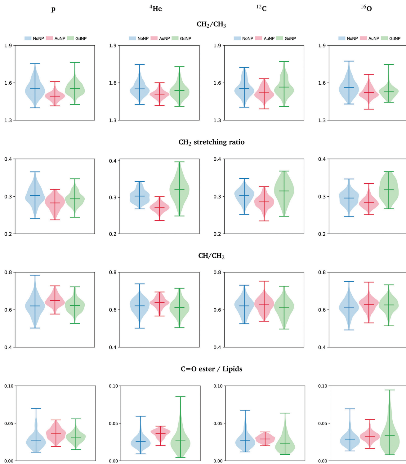
Fig. 9 All ions (p, ^4\text{He} , ^{12}\text{C} , ^{16}\text{O} ; from left to right); 20 GyRBE. SR-FTIR results on the radiosensitization mechanisms of GdNP and AuNP in charged particle therapy. Distribution of the relative intensities of the \text{CH}_2/\text{CH}_3 , \text{CH}_2 stretching ratio, \text{CH}/\text{CH}_2 and \text{C}=\text{O} ester/lipids spectral band ratios in the absence (NoNP; blue) and in the presence of AuNP (red) and GdNP (green). See Table 1 for more information on the bands assignment.
