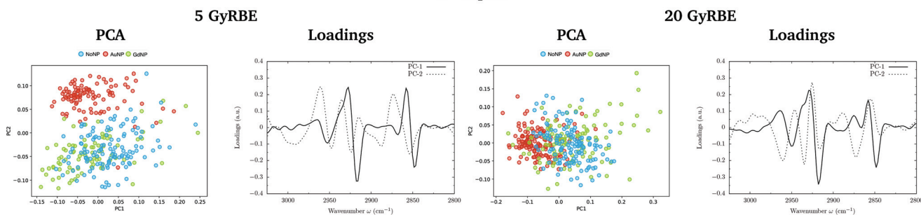
Fig. 4 Oxygen beam irradiations. SR-FTIR results on the radiosensitization mechanisms of GdNP and AuNP in charged particle therapy. The PCA scores and the loading plots are presented in the fingerprint (1800–950 \text{cm}^{-1} , top) and lipids (3025–2800 \text{cm}^{-1} , bottom) spectral regions in the absence (NoNP; blue) and in the presence of AuNP (red) and GdNP (green) for 5 GyRBE (left) and 20 GyRBE (right).
