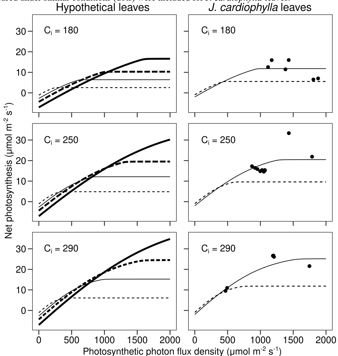
Figure 3: Comparison of simulated light response curves of net photosynthesis obtained using the parameterizations derived in this study for Sonoran Desert species (solid lines) and parameterizations for the shrub functional type from Kattge et al. (2009) (dashed lines). Simulations were performed for hypothetical leaves with high N_{\text{area}} (4.5 g N m -2 , thick lines) and low N_{\text{area}} (1 g N m -2 , thin lines) and for J. cardiophylla leaves, under high leaf temperatures (37 °C) and acclimated to typical July temperatures of our study locations. We used three levels of intercellular CO 2 concentration ( C_i ) corresponding to typical values found at low and high stomatal conductance: 180 \mu\text{mol mol}^{-1} for stomatal conductances of 0.1-0.2 mol m -2 s -1 , and 290 \mu\text{mol mol}^{-1} for stomatal conductances of 0.6-1 mol m -2 s -1 , respectively). Also included was a typical intercellular CO 2 concentration for C 3 species (250 \mu\text{mol mol}^{-1} ) which is about the mean value of our data (Lambers et al. 2008). Data measured under similar conditions (dots) were included for J. cardiophylla leaves.
