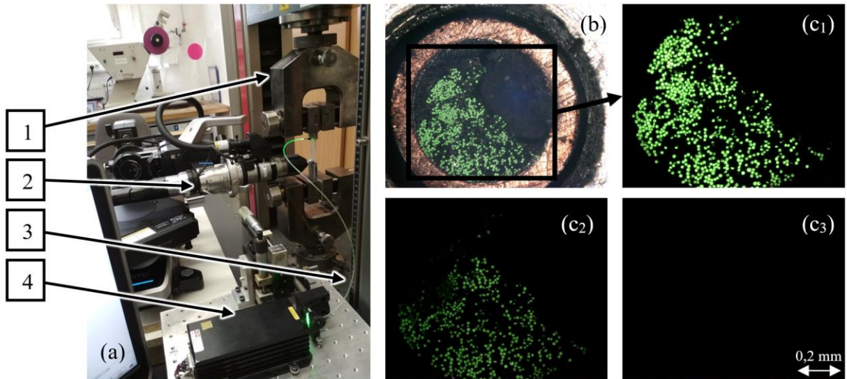
Fig. 3 Measurement layout (a) and the microscopy images of the end of the fiber bundle before loading (b) and at the “moment” of breakage (c 1 , c 2 , c 3 ) (there was \sim 0.07 second between the frames) (1 – upper clamp of the tensile tester, 2 - digital microscope, 3 - optical cable, 4 - light source)
