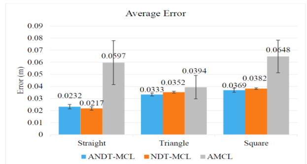
Figure 10. The average error and standard deviation produced by each of the algorithms
