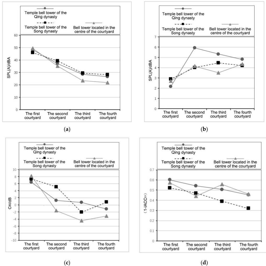
Figure 9. Diagrams of the effects of bell tower position on courtyard sound fields. (a) Variation in SPL(A). (b) Variation in the standard deviation of SPL(A). (c) Variation in C 80 . (d) Variation in (1-IACC E3 ).
