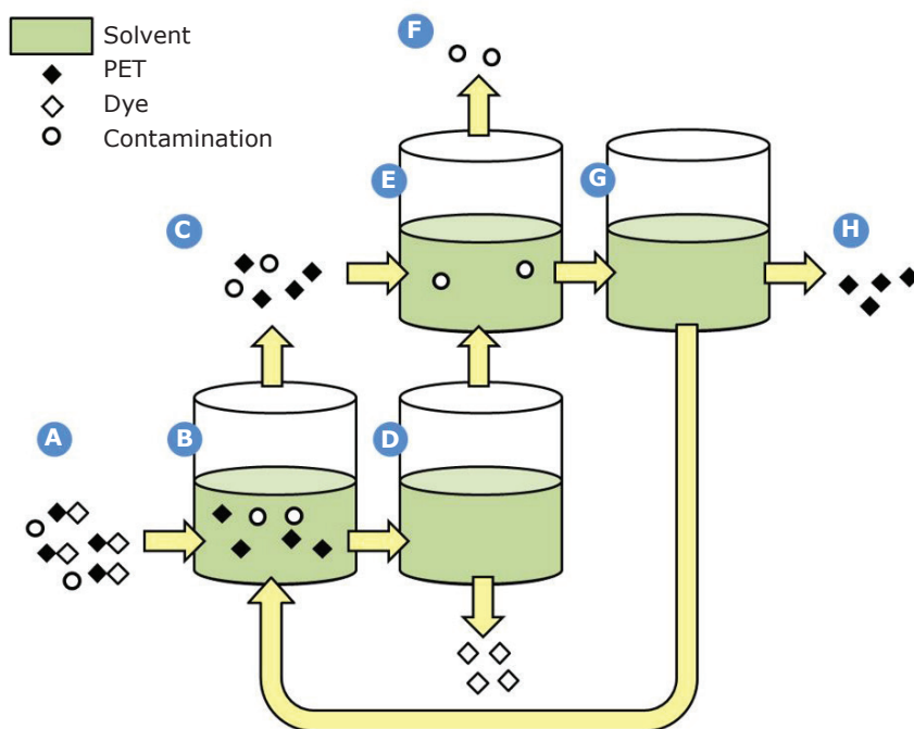
Fig. 1. Simplified schematic of the Worn Again PET recycling process; A contaminated and dyed PET collected; B dye dissolved (low temperature); C contaminated PET filtered; D dye solution removed and solvent reclaimed; E PET dissolved (high temperature); F contamination filtered; G PET solution cooled to precipitate PET and reclaim solvent; H recycled PET
