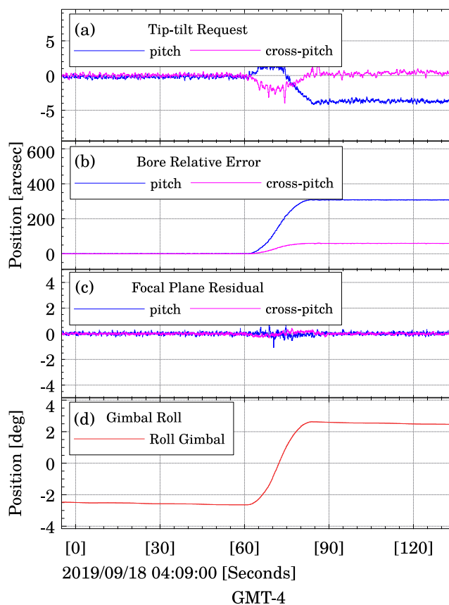
FIG. 7. A target re-acquisition and continuous target tracking during simultaneous roll and fine pitch gimbal resets; gimbal frames track in unison about the FPSC target star while the FGS attenuates perturbations at the 2–4 in. level (a) down to <0.2 in. (c) during the reset, the boresight star camera centroids (b) show a mean shift post-reset due to an offset pointing vector with the FPSC(s) as the roll gimbal is slewing (d); the maximum sky-equivalent throw of the FGS in pitch and cross-pitch is 12.61 in. and 8.92 in., respectively.
