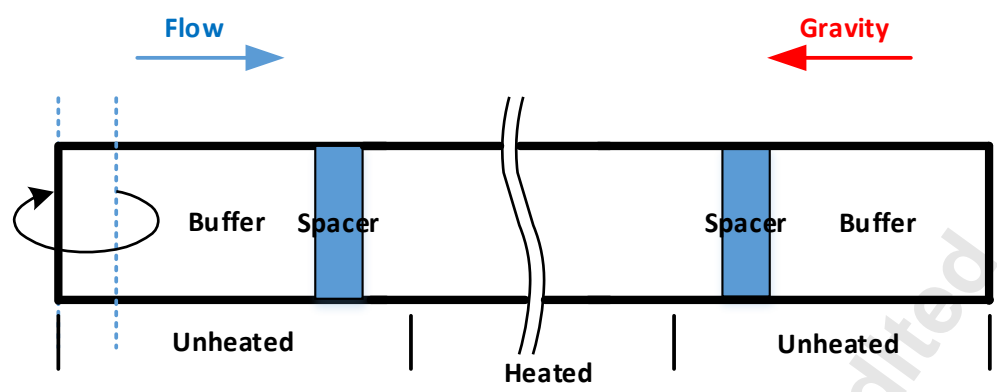
Fig. 8 Schematic of the numerical model.
