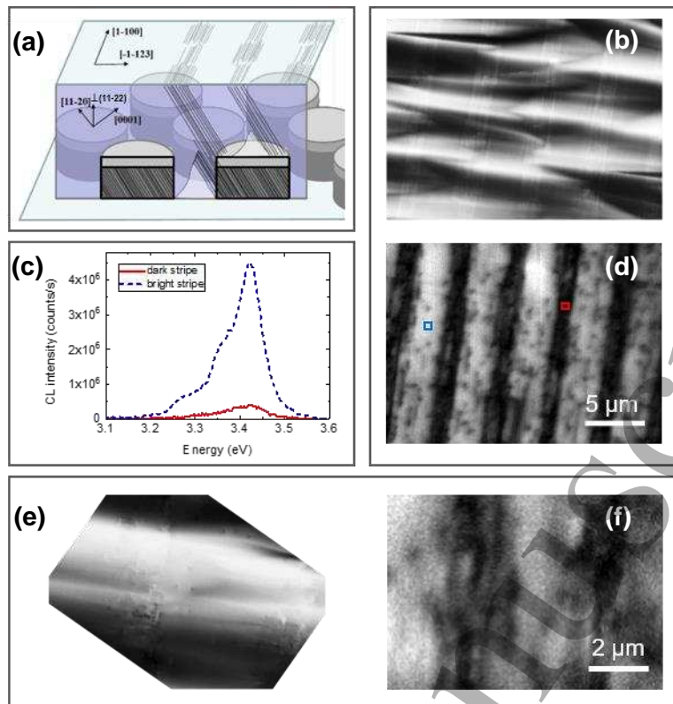
Fig. 7. (a) Schematic of semi-polar GaN microrod template and overgrowth, indicating the distribution of stacking faults on the surface of the sample and the crystallographic directions (b) ECCI micrograph revealing basal-plane stacking faults (c) Example CL spectra from a dark stripe and a bright stripe, respectively. The boxes on Fig 6 (d) indicate where the spectra were extracted from the CL dataset. (d) Integrated CL intensity image of the GaN near band edge (NBE) emission (3.15-3.50 eV) on the same scale as (e) but not from the same area. (e) Higher resolution ECCI micrograph revealing dislocations (f) Integrated CL intensity image of the GaN near band edge (NBE) emission (3.15-3.50 eV) on the same scale as (e) but not from the same area. From [48] under Creative Commons Attribution (CC BY) license: http://creativecommons.org/licenses/by/4.0/
