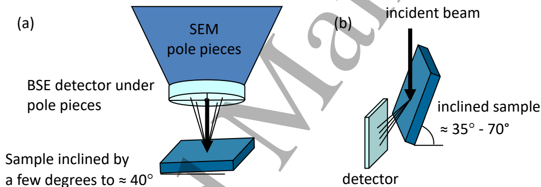
Fig. 1. Illustration of the (a) backscatter and (b) forescatter geometries for acquisition of ECCI micrographs [reproduced from 31].
