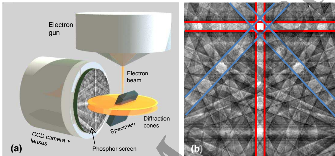
Fig. 3. (a) Illustration of the EBSD detection geometry and a conventional EBSD detector,
