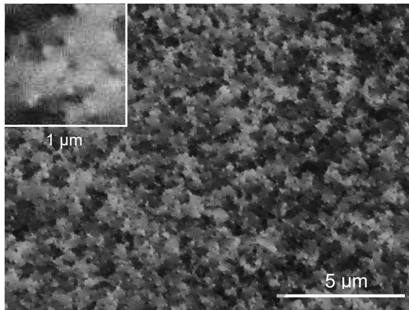
Fig. 4. ECCI micrograph from AlGaIn thin film. Inset shows dislocation “spots” at higher magnification. Adapted from [48] under Creative Commons Attribution (CC BY) license: http://creativecommons.org/licenses/by/4.0/
