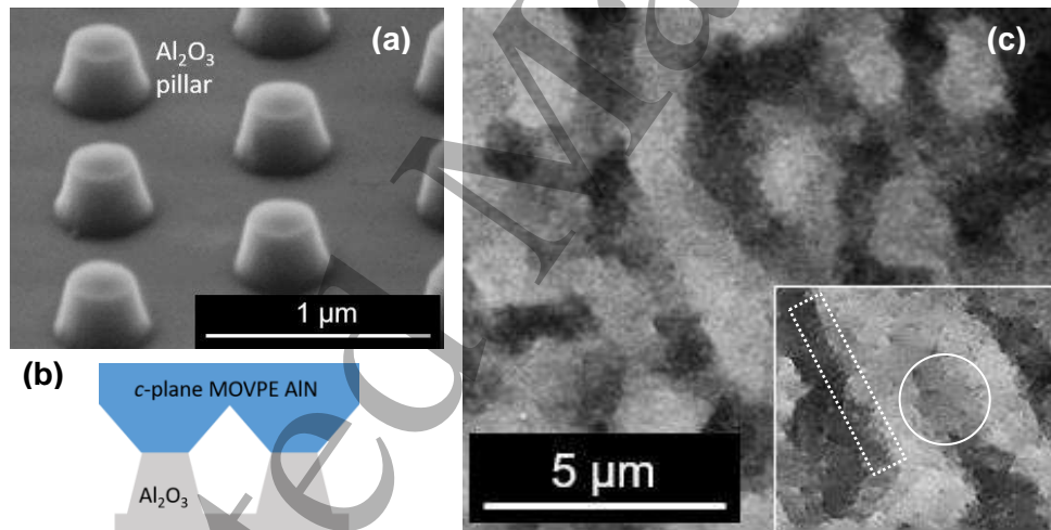
Fig. 5. (a) Secondary electron image of nPSS, (b) schematic of overgrowth of AlN on nPSS and (c) ECCI micrograph from an AlN thin film, inset is on same scale but with higher resolution. Adapted from [48] under Creative Commons Attribution (CC BY) license: http://creativecommons.org/licenses/by/4.0/
