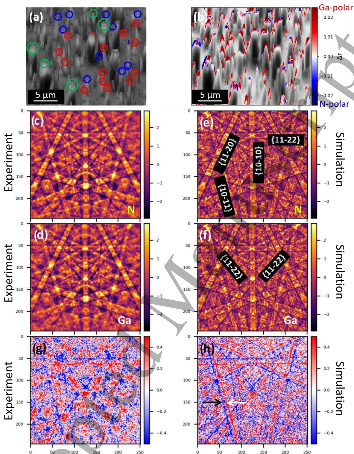
Fig. 9 (a) backscattered electron image of the area of the sample investigated by EBSD. The NWs circled in blue are N-polarity, those circled in red are Ga-polarity and those circled in green are mixed polarity. (b) Cross-correlation difference map indicating N-polarity in blue and Ga-polarity in red, overlaid on a BSE intensity image derived from the raw EBSPs. (c) Experimental EBSP from the point marked with a blue cross from a GaN NW with N-polarity, (d) experimental EBSP from the point marked with a red cross from a GaN NW with Ga-polarity. (e, f) Simulated patterns for N and Ga polarity, respectively. (g) Normalised intensity difference image of the experimental EBSPs (from (c) and (d)), and (h) normalised intensity difference image of simulated EBSPs (from (e) and (f)). The white arrow points to {10-11} and the black arrow points to {10-1-1}. Adapted from [40] under Creative Commons Attribution (CC BY) license: http://creativecommons.org/licenses/by/4.0/
