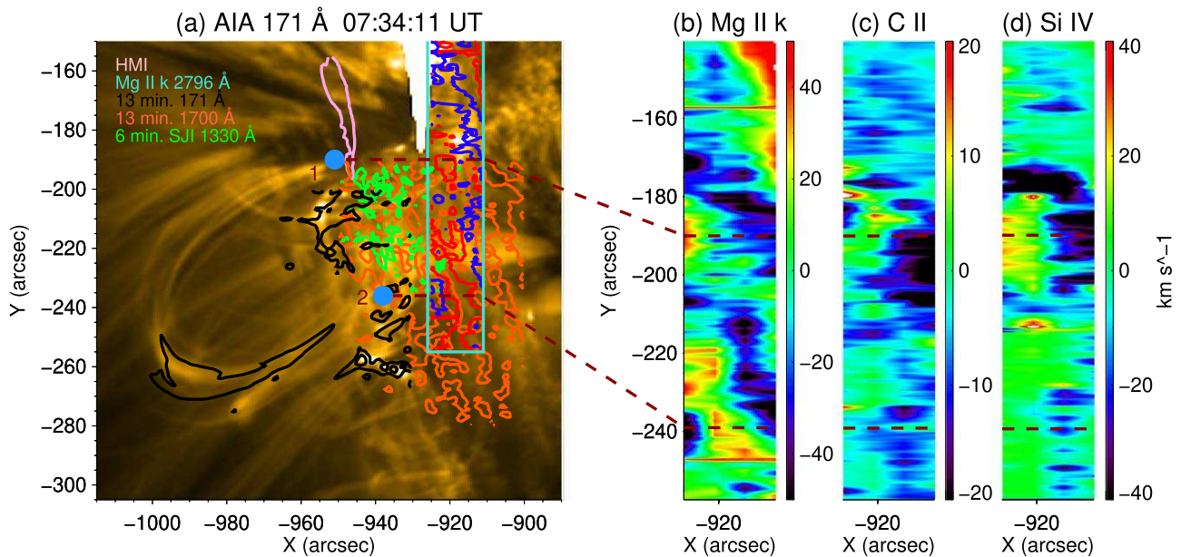
Figure 5. (a) Coronal loops of AR 11967 as seen in SDO/AIA 171 Å and spatial location of the oscillations found in the loops. The pink contour represents the sunspot position seen from the HMI instrument (Scherrer et al. 2011) and blue filled circles show the position of the endpoints of the loops. Oscillations of 13 minutes observed in SDO/AIA 171 Å and 1700 Å are indicated by the black and orange contours, respectively. We also show, for comparison, the 6 minute oscillations as detected in SJI-1330 Å by green contours. The aquamarine box encloses the FOV of the dopplergram for the Mg II k 2796 Å spectral line. The blue color means negative velocities showing up-flow, and red represents the opposite. The dashed lines connect the position of the endpoints with the dopplergram overlapped in panel (a) and with more details in panel (b). Panels (c) and (d) show dopplergrams for C II 1336 Å and Si IV 1403 Å, respectively.
