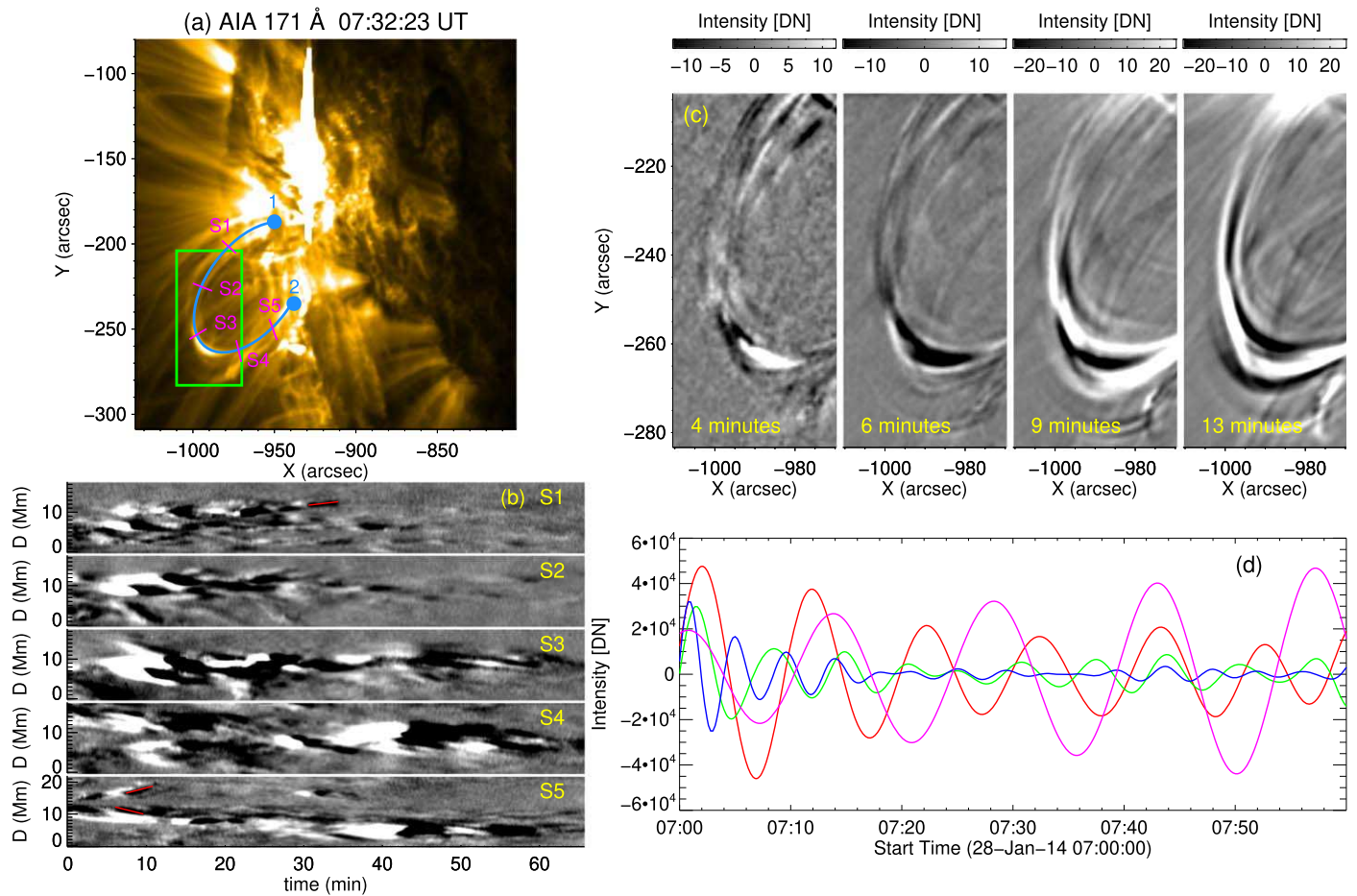
Figure 3. Oscillations found in the top of the coronal loops observed in SDO/AIA 171 Å. (a) EUV snapshot of the coronal loops as observed in SDO/AIA 171 Å passband. The loop shape and its endpoints are shown in blue color. (b) Distance–time maps made for each purple slit traced across the loop in panel (a). Disturbance speed was calculated over the slits S1 and S5, which are represented by red lines. (c) Filtered intensity maps for oscillations of 4, 6, 9, and 13 minutes seen in the loop-tops region shown in (a). (d) Filtered integrated intensity variation as a function of time for the maps shown in (c). Lines blue, green, red, and purple correspond to oscillations of 4, 6, 9, and 13 minutes, respectively.
