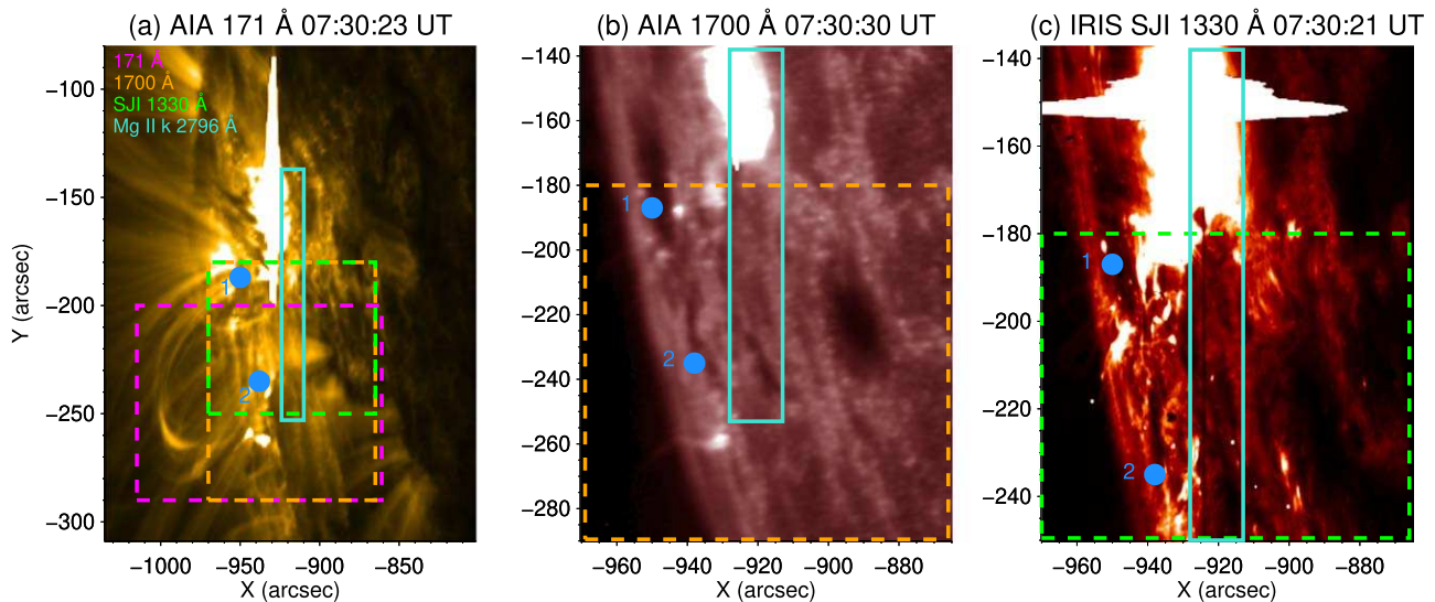
Figure 1. Image of AR 11967 on 2014 January 28 at about 07:30 UT observed in (a) SDO/AIA 171 Å (b) SDO/AIA 1700 Å and (c) IRIS SJI 1330 Å wavelength passbands. The orange dashed box on the left panel denotes the region of interest (ROI) of SDO/AIA 1700 Å images analyzed. The IRIS SJI 1330 Å data is available for a shorter region and is denoted by the green dashed box. The aquamarine box represents the region of interest (ROI) of spectral data (SG). The ROI chosen for the subsequent analysis includes the green, orange, and purple dashed lines. We indicate the position of the endpoints of the loops, as inferred from the 171 Å images, by the blue circle. Endpoint 1 is very close to the sunspot shown in 1700 Å (panel (b)).
