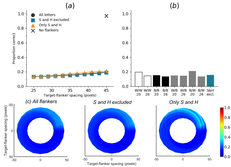
Figure S1: Accuracy of letter identification of the first randomly initialised small 5-layer convolutional network with single flankers ('SimpleNet 1'). Training and testing was done without acuity loss. Average accuracy without flankers was 97.16%.
