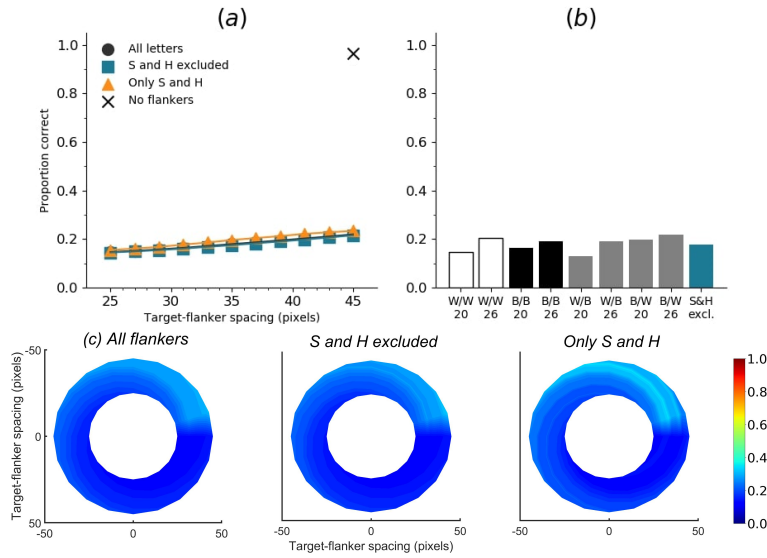
Figure S4: Accuracy of letter identification of the fourth randomly initialised small 5-layer convolutional network with single flankers ('SimpleNet 4'). Training and testing was done without acuity loss. Average accuracy without flankers was 96.59%.
