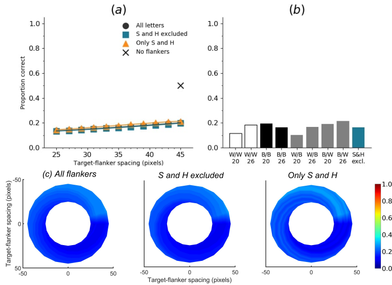
Figure S6: Accuracy of letter identification of the randomly initialised small 5-layer convolutional network with single flankers ('SimpleNet'). A total of five independent training sessions and test sessions are combined in this figure. Training of all five models in this figure was done without acuity loss, and testing was done with acuity loss. Average accuracy without flankers was 50.02%.
