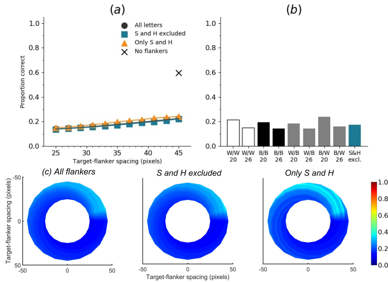
Figure S11: Accuracy of letter identification of the fifth randomly initialised small 5-layer convolutional network with single flankers ('SimpleNet 5'). Training was done without acuity loss, and testing with acuity loss. Average accuracy for acuity-reduced data without flankers was 59.51%.
