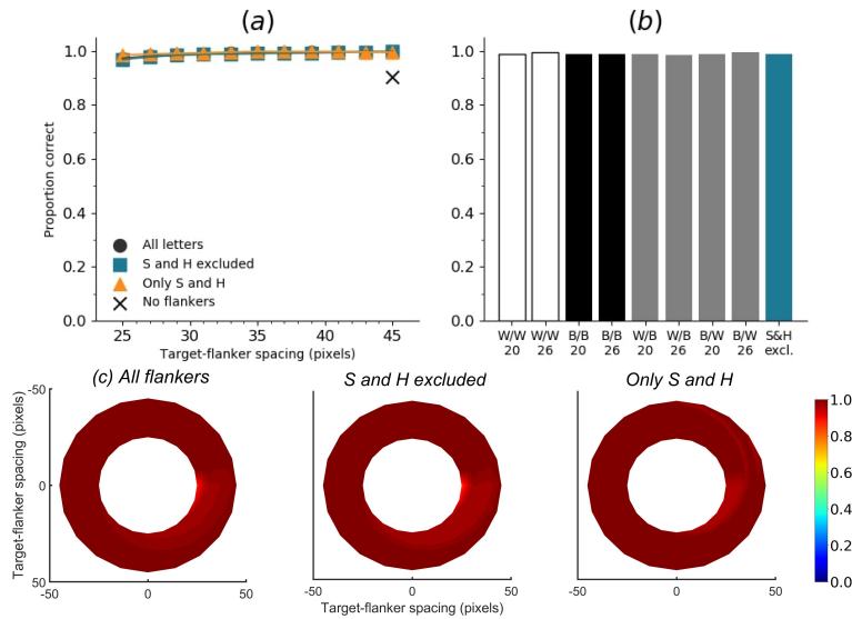
Figure S16: Accuracy of letter identification of the DenseNet-121 with random weight initialisation and no acuity loss with single flankers. Model base accuracy was 90.25%. Note that accuracy is increased by adding a flanker—the only position that does not exhibit this behaviour is the same position that causes the most crowding in almost all of our other tests.
