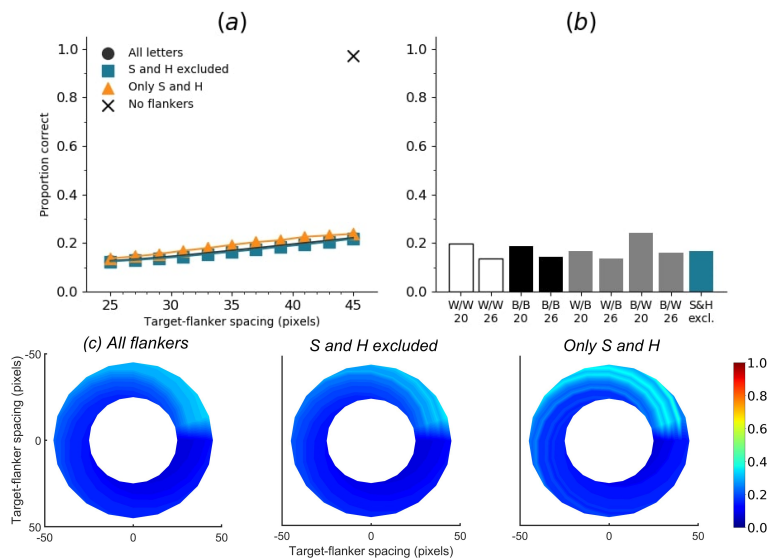
Figure S5: Accuracy of letter identification of the fifth randomly initialised small 5-layer convolutional network with single flankers ('SimpleNet 5'). Training and testing was done without acuity loss. Average accuracy without flankers was 97.22%.
