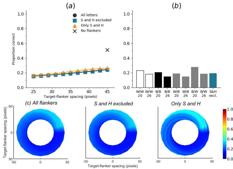
Figure S10: Accuracy of letter identification of the fourth randomly initialised small 5-layer convolutional network with single flankers ('SimpleNet 4'). Training was done without acuity loss, and testing with acuity loss. Average accuracy for acuity-reduced data without flankers was 51.21%.
