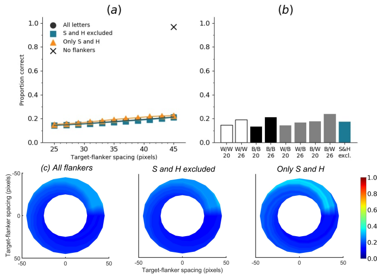
Figure 4: Accuracy of letter identification of the randomly initialised small 5-layer convolutional network with single flankers ('SimpleNet'). A total of five independent training sessions and test sessions are averaged in this figure. Results of individual runs are shown in Supplementary Figures S1-S5. Training and testing of all five models in this figure was done without unaltered images. Average accuracy without flankers was 96.97, as shown in panel (a)%. The letters S and H are excluded in (c) middle and shown exclusively in (c) right, as the network had not seen the letters in testing. We also tested the SimpleNets with acuity-reduced stimuli—Figure S6 shows the averaged results, and Figures S7-S11 show individual models' results. We found that accuracy reached near-chance levels (12.5%), and as such little can be inferred from these results.
