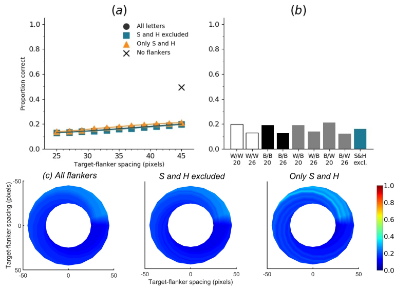
Figure S7: Accuracy of letter identification of the first randomly initialised small 5-layer convolutional network with single flankers ('SimpleNet 1'). Training was done without acuity loss, and testing with acuity loss. Average accuracy for acuity-reduced data without flankers was 49.33%.
