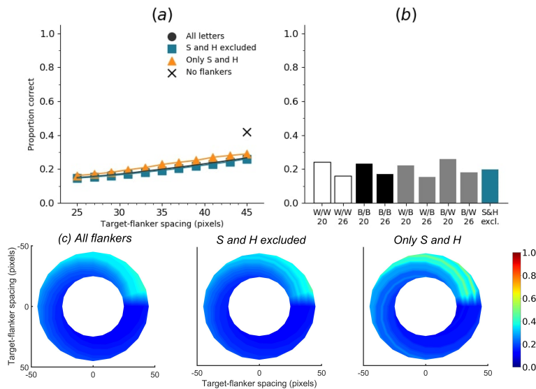
Figure S9: Accuracy of letter identification of the third randomly initialised small 5-layer convolutional network with single flankers ('SimpleNet 3'). Training was done without acuity loss, and testing with acuity loss. Average accuracy for acuity-reduced data without flankers was 42.06%.
