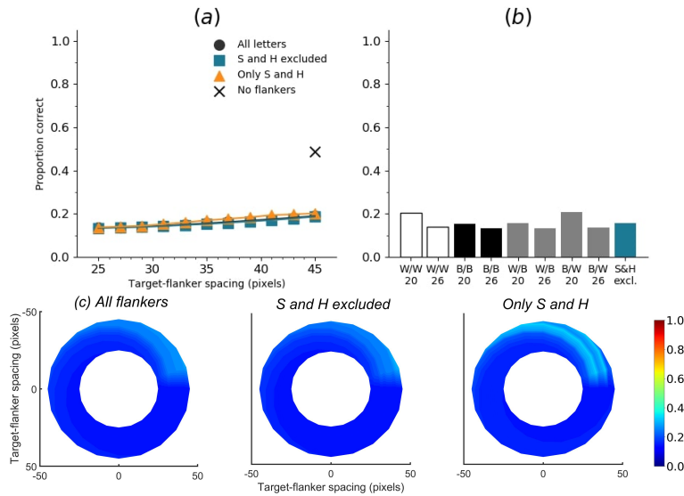
Figure S8: Accuracy of letter identification of the second randomly initialised small 5-layer convolutional network with single flankers ('SimpleNet 2'). Training was done without acuity loss, and testing with acuity loss. Average accuracy for acuity-reduced data without flankers was 48.91%.
