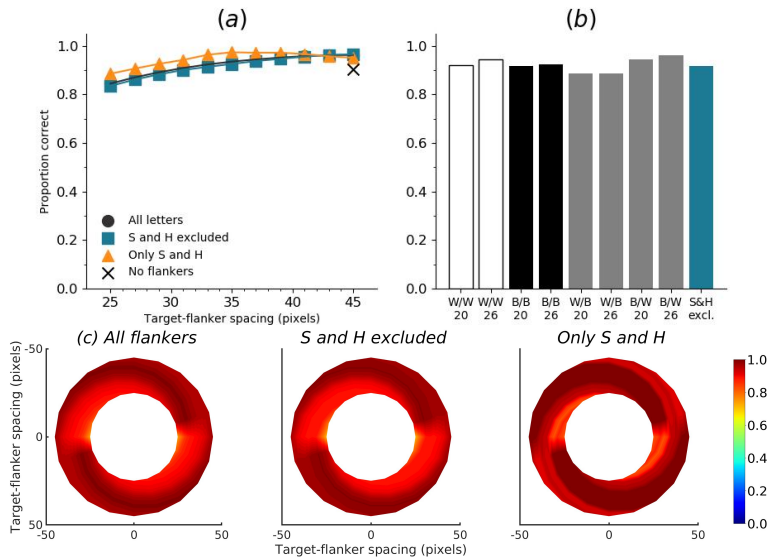
Figure S17: Accuracy of letter identification of the DenseNet-121 by distance and colour for pair flankers with random weight initialisation and no acuity loss. Accuracy without flankers was 90.25%. Note that as this is the same model as presented in Figure S16—some positions of flankers also increase accuracy.
