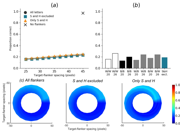
Figure S3: Accuracy of letter identification of the third randomly initialised small 5-layer convolutional network with single flankers ('SimpleNet 3'). Training and testing was done without acuity loss. Average accuracy without flankers was 97.25%.
