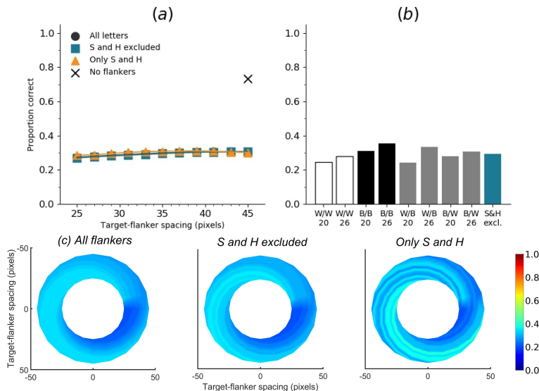
Figure 5: Accuracy of letter identification for the ILSVRC-initialised VGG-16 model with single flankers. Even though the accuracy for unflanked targets in the VGG-16 was lower than for the SimpleNets, it appears to be more robust to clutter; that is, flanked performance is higher. Nevertheless, the general pattern of crowding remains the same. VGG-16 accuracy without flankers was 73.46%.
