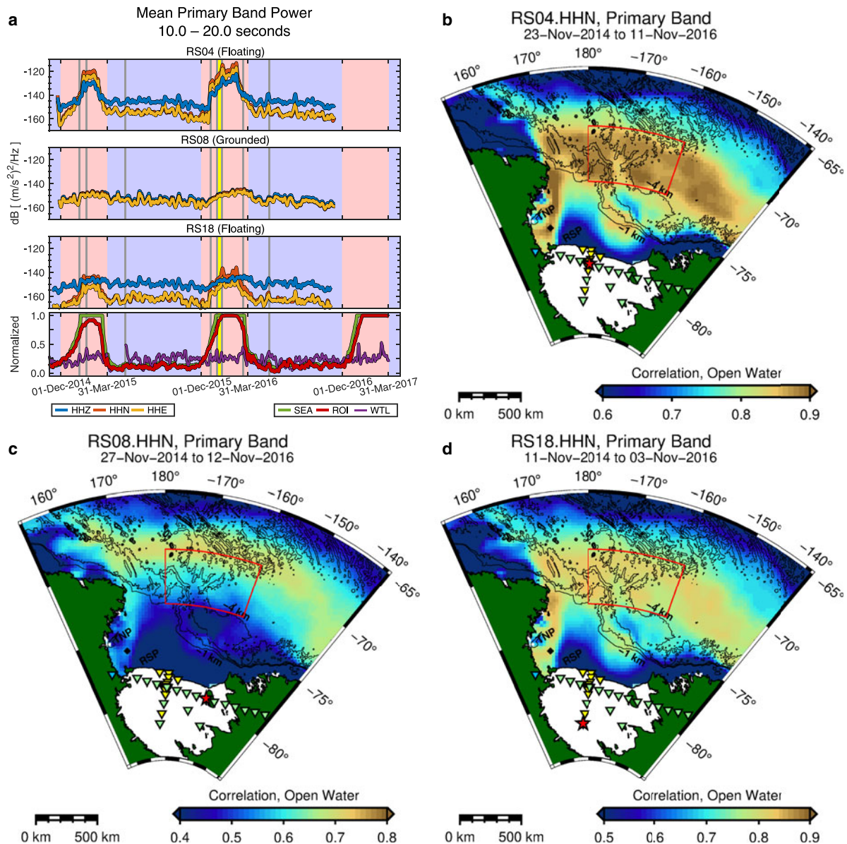
Fig. 5. (a) Daily average primary band powers for vertical (HHZ), north (HHN) and east (HHE) seismometer channels, compared to median open water concentration for the entire mapped region (SEA), the mean open water concentration for the red-bounded region-of-interest (ROI) and the mean daily wind speed measured at Franklin Island (WTL). Wind velocity has been normalized to 20 \text{ m s}^{-1} . Primary band powers and wind velocity were smoothed with a \pm 5 day moving average; open water concentrations were not smoothed. The vertical yellow band marks the 10 January to 21 January 2016 RIS melt event; the gray vertical bars mark wind events that correlate with elevated spectral band powers. Red and blue backgrounds indicate summer and winter months, respectively. (b–d) Pearson's correlation coefficients for daily mean primary band north component power and daily open water concentration at each cell. Both time series were smoothed with a \pm 1 day moving average before correlation. Spatial distributions for vertical and east channels are similar. The red ROI overlaps a near-central portion of the Ross Gyre.
