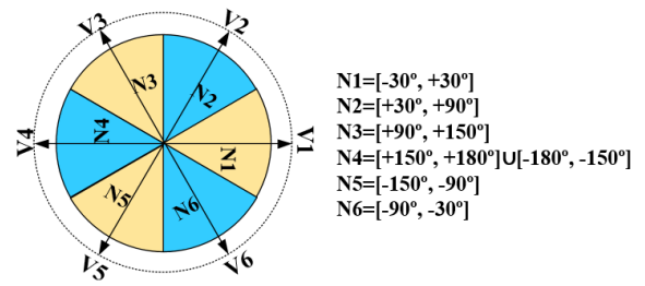
Fig. 16. Zones arrangement for the proposed converter.
