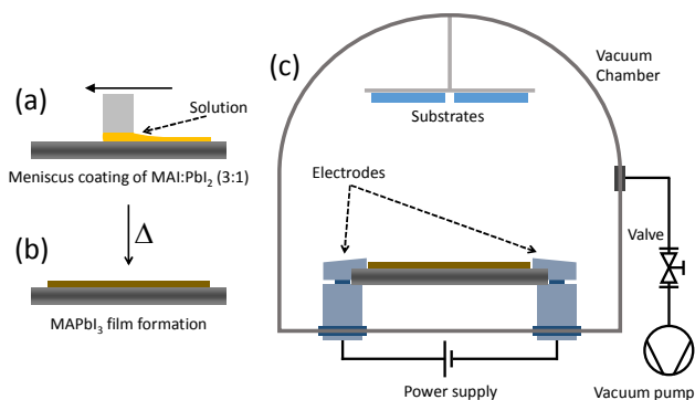
Fig. 1. Process flow for the deposition of hybrid organic-inorganic perovskite thin films via flash evaporation. (a) The precursor solution is spread onto a tantalum foil via meniscus coating and (b) annealed to obtain a polycrystalline \text{CH}_3\text{NH}_3\text{PbI}_3 film. The coated tantalum sheet is then transferred to a vacuum chamber (c) where the hybrid perovskite is evaporated onto the desired substrate.
