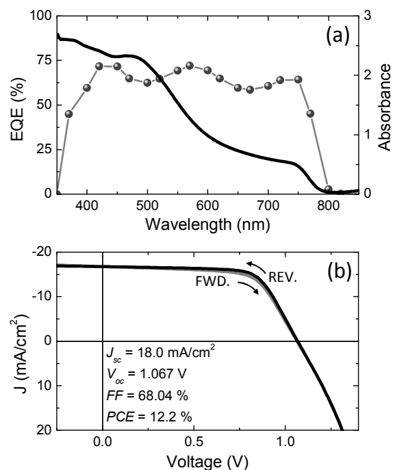
Fig. 3 (a) EQE (symbols) and optical absorption (line) in the UV-visible region for a planar perovskite solar cell and its active layer, respectively, deposited by flash evaporation. (b) J-V curve in forward (FWD.) and reverse (REV.) bias for a device under illumination with the structure ITO/PEDOT:PSS/PolyTPD/MAPbI 3 /PCBM/Ba/Ag. The scan rate in both bias direction was 0.1 V/s.
