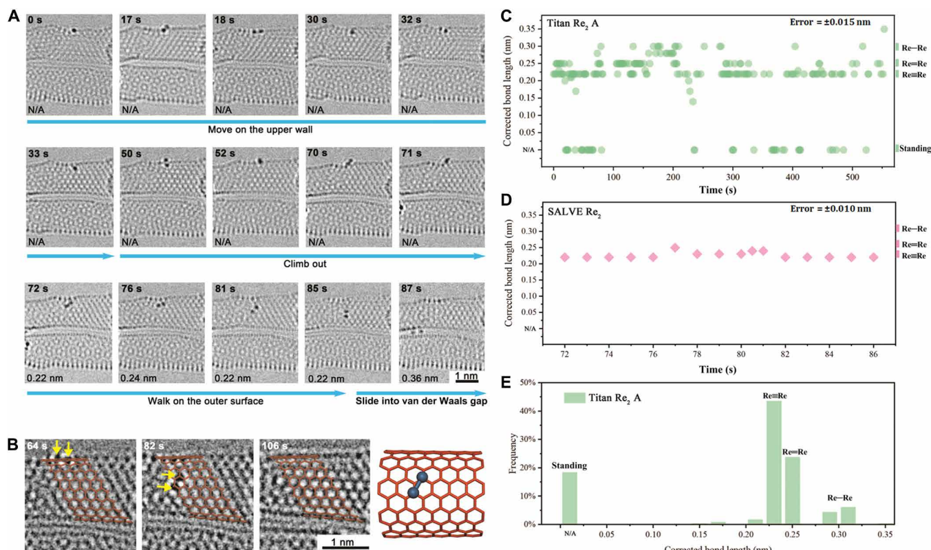
Fig. 2. Changes in Re–Re bond length over time. (A) Time-series AC-HRTEM images (80 kV) (unprocessed data) of the first stage of movie S2 acquired by the SALVE TEM. At this stage, the dirhenium molecule moves at a defect site on the SWNT, climbs out from the defect, and then slides into the vdW gap between two parallel SWNTs. The corrected Re–Re bond length of each frame is presented; error is \pm 0.010 nm. (B) Selected frames with adjusted high contrast from movie S2 for analyzing the atomically precise position of the dirhenium molecule when it is drifting along the outer surface of host SWNT. The position of the Re atoms are indicated by yellow arrows. The AC-HRTEM images are partially covered by the model of an SWNT with chirality of (10, 10). The simulated structure shows the position of dirhenium molecule in the frame of 82 s. (C) Corrected bond length changing of the right dirhenium molecule in movie S1 (Titan Re 2 A); error is \pm 0.015 nm. (D) Corrected bond length of the dirhenium molecule drifting along the outer wall of SWNT in movie S2 (SALVE Re 2 ); error is \pm 0.010 nm. (E) The histogram shows the count frequencies of the different bond lengths of Titan Re 2 A (0 to 553 s).
