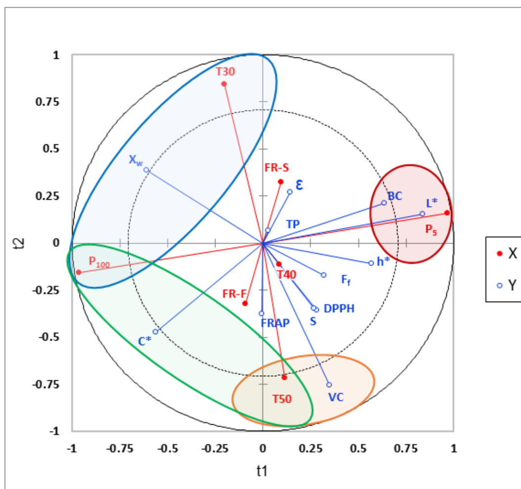
Figure 1. PLS-R projections of freeze-dried orange puree at a range of pressure, temperature and rate of freezing conditions. The dependent variables (X) are projected in red and the qualitative explanatory variables (Y) are projected in blue. The variables Y significantly correlated with a specific dependent variable are circled in red, blue, orange and green. Variables X: T30, T40, T50: shelf temperature applied during freeze-drying at 30, 40 and 50 °C, respectively; P 5 and P 100 : working
