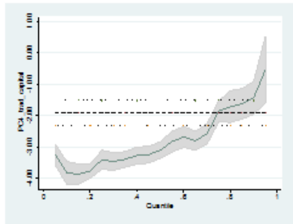
Figure 2.D.: PC4_trad_capital
