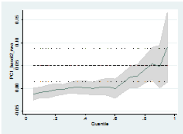
Figure 1.A. PC1_basel2_rwa
