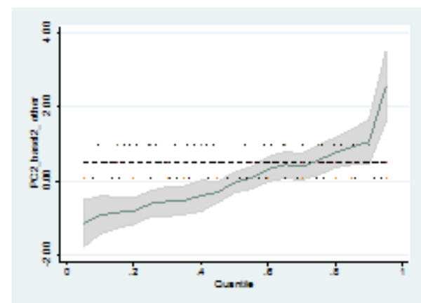
Figure 2.B. PC2_basel2_other
