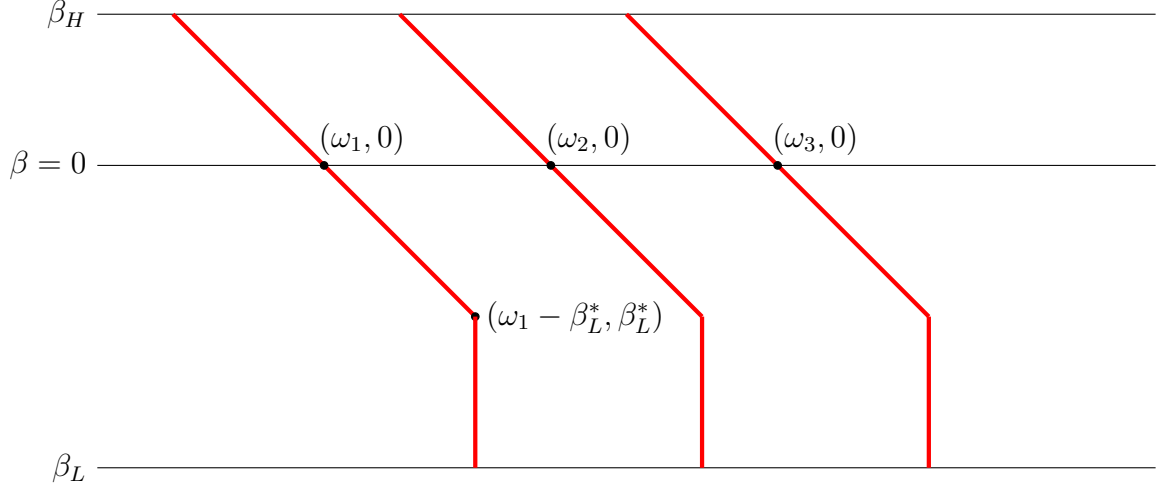
Figure 4: Unbounded Uniform Model, -\beta_L > \beta_H .
