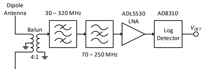
Fig. 3. RF front-end electronics.
