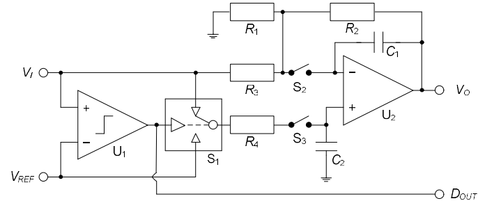
Fig. 9. Proposed sample-hold folding amplifier.
