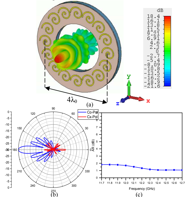
Fig. 6. 16-element circular sub-array (a) 3D radiation pattern (b) 2D radiation pattern (c) axial ratio (broadside radiation)
