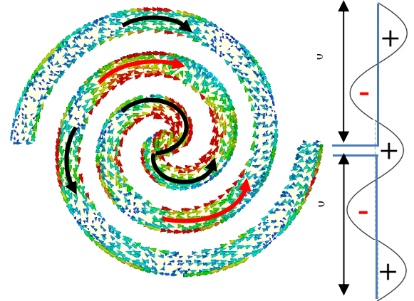
Fig. 3. Current distributions at the central frequency.
