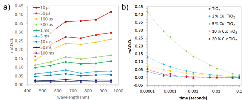
Figure 4. (a) Transient absorption spectra at select times for the 5% Cu-doped TiO 2 thin film. (b) Recombination kinetics at 950 nm for all samples, where the dashed lines represent a fit to a power law decay model [ f(t) = a \cdot t^b , where t is the time and a and b are variables].
