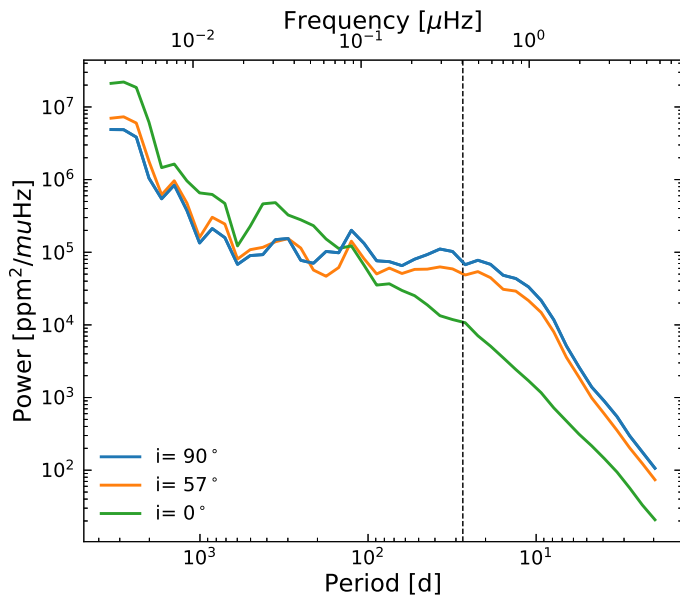
Fig. A.3. Power spectra of the solar brightness variations for Strömgren y for different inclinations.
