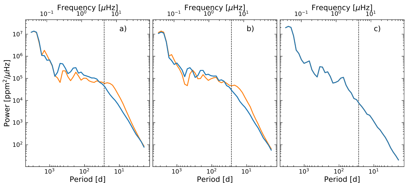
Fig. 8. Comparison of the power spectra of the solar brightness variations in the Kepler passband, with and without taking the solar rotation into account (orange and blue, respectively). Panel a) shows 90° inclination, b) 57° and c) 0°. The vertical dashed black lines indicates the synodic solar rotation period at 27.3 days.
