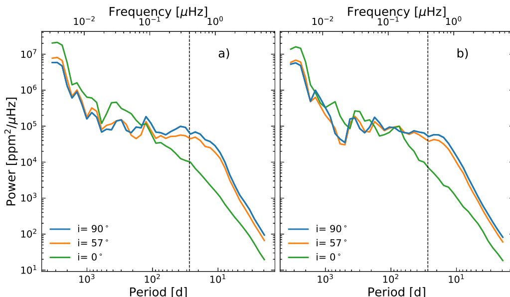
Fig. 6. Power spectra of solar brightness variations in the Kepler passband with different inclinations and two different cycles. Panel a) shows cycle 19 and panel b) cycle 22. The vertical dashed black lines indicate the synodic solar rotation period at 27.3 days.
