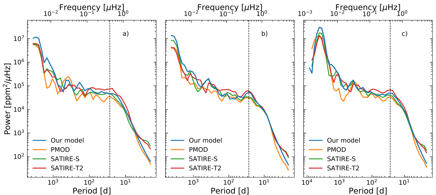
Fig. 1. Comparison of the power spectra of solar brightness variations produced by our model to those given by the PMOD-composite as well as SATIRE-S and SATIRE-T2 models for cycle 22 (panel a) and cycle 23 (panel b) and the combined timeseries (panel c). The vertical dashed black line indicates the synodic solar rotation period of 27.3 days.
