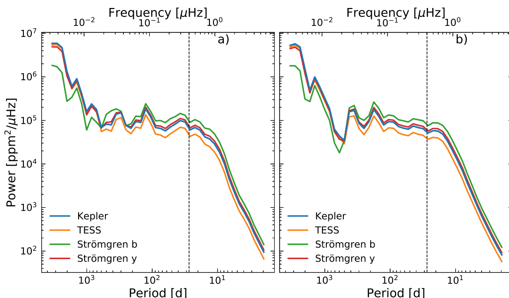
Fig. 5. Power spectra of solar brightness variations in different filter systems for different cycles as observed from the ecliptic. Panel a) shows cycle 19, panel b) cycle 22. The vertical dashed black line indicates the synodic solar rotation period at 27.3 days.
