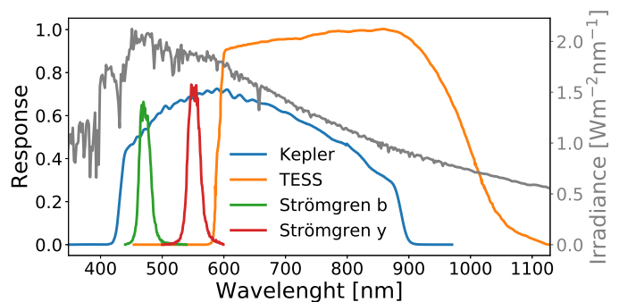
Fig. 4. Response functions of the different filter systems used in this work. The quiet-Sun irradiance as used by SATIRE is shown in grey.
