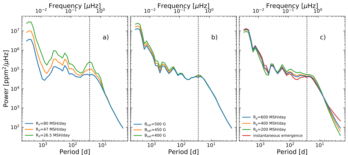
Fig. 2. Effect of the different parameters of the model on the brightness variations. Panel a) shows the effect of the decay rate R_d on the spot component only, panel b) the effect of B_{sat} on the total power spectrum and panel c) the effect of different growth rates R_g on the total power spectrum compared to not having the spot growth included as depicted by the red curve. R_d and R_g are in units of \text{MSH day}^{-1} . The vertical dashed black line indicates the synodic solar rotation period at 27.3 days.
