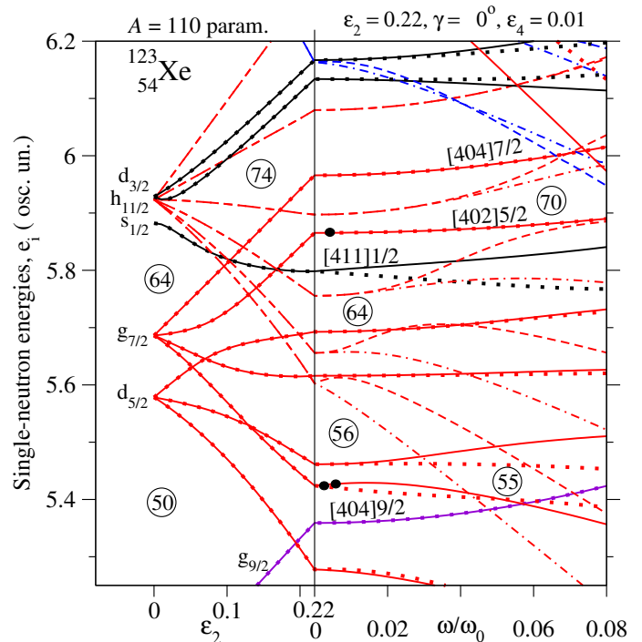
FIG. 1. (Color online) Single-particle neutron energies at a prolate shape as a function of the deformation parameter, \epsilon_2 , (left part) and as a function of the rotational frequency at \epsilon_2 = 0.22 (right part). Note that, for a larger quadrupole deformation and/or rotational frequency, it will be advantageous to create proton holes in the g_{9/2} shell of the Z=50 core, leading to configurations of larger collectivity [17, 22–24]. Negative-parity orbitals are drawn by dashed lines while dots are used for signature \alpha = -1/2 orbitals, i.e. full lines are used for (\pi, \alpha) = (+, +1/2) , dots for (+, -1/2) , dashed lines for (-, +1/2) and dashed-dotted lines for (-, -1/2) .
