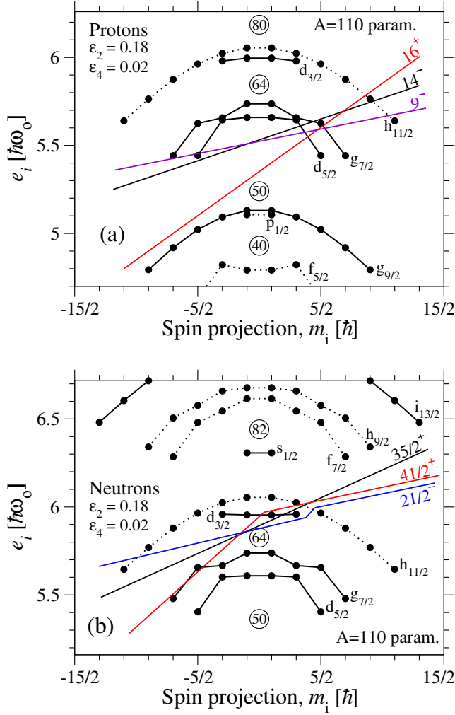
FIG. 9. (Color online) Calculated single-particle energies, e_i , as a function of the spin-projection quantum number, m_i , calculated at \varepsilon_2 = 0.18 , \gamma = 60^\circ , and \varepsilon_4 = 0.020 : (a) for protons and (b) for neutrons. Some low-lying aligned configurations are defined by ‘straight-line Fermi surfaces’ [13], where the orbitals below the lines are occupied and the total spin is obtained as the sum of the projections m_i below the lines.
