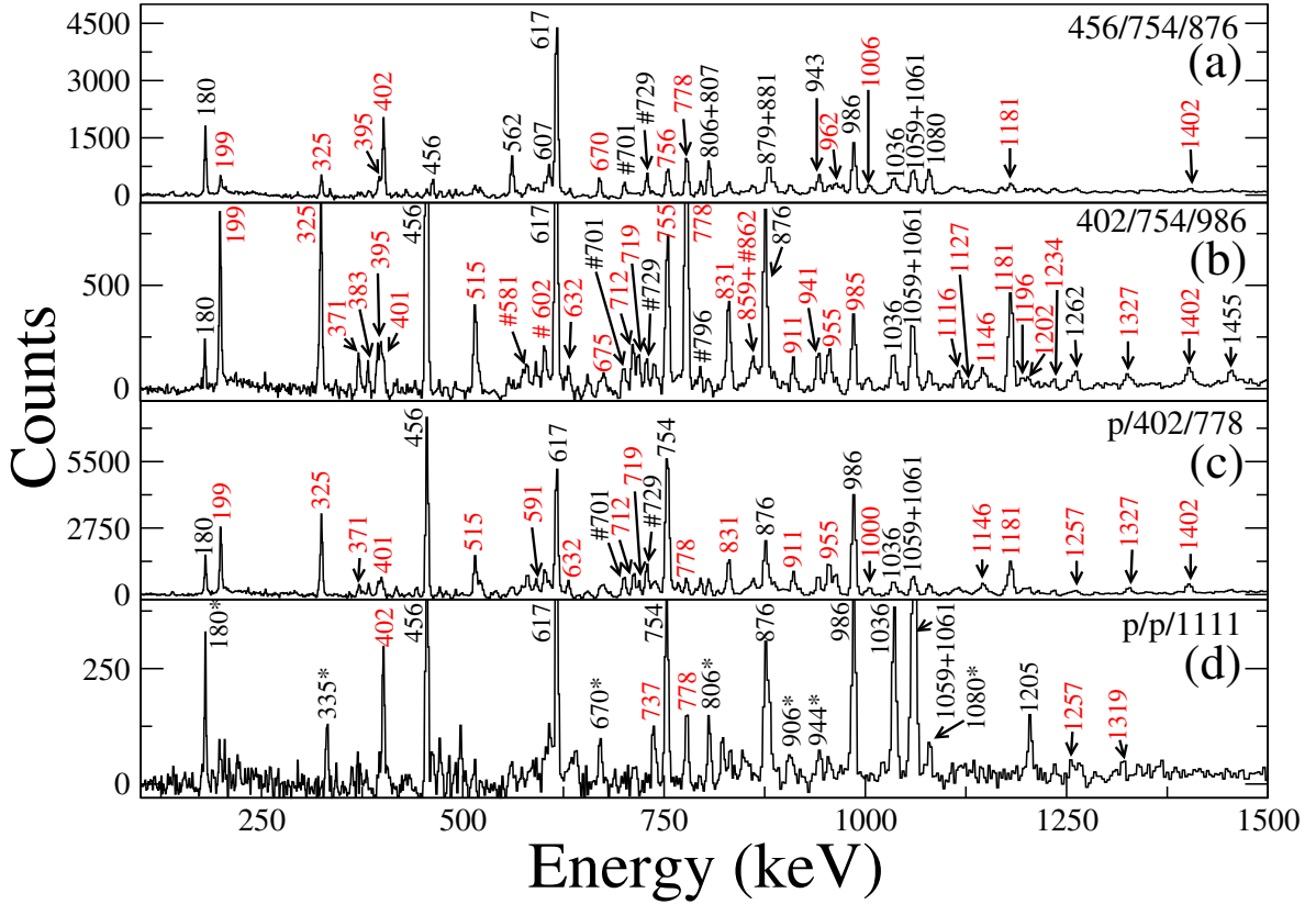
FIG. 5. (Color online) Background-subtracted summed triple-gated \gamma -ray coincidence spectra. Panel (a): spectrum obtained with triple gates on 456-, 754-, and 876-keV transitions. The transitions of band 6 and its decay-out transitions are displayed. Panel (b): The presence of second 401-, 755-, and 985-keV \gamma rays can be seen in spectrum with triple gates on 402, 754, and 986 keV. Panel (c): quadruple coincidence of list ‘p’ of 456-, 617-, 754-, and 876-keV transitions of band 9, and the 402- and 778-keV transitions. The transitions of bands 7 and 8 can be seen in this spectrum. Panel (d): quadruple-coincidence spectrum with two gates on \gamma rays from list ‘p’, and the 1111-keV transition of band 9. The new transitions of band 9 and the 737-keV transition linking bands 7 and 8 to band 9 are displayed. The \gamma rays marked by # belong to bands 1, 2, and 3. The transitions marked by * are from bands 12 and 13 of ^{123}\text{Xe} . The new transitions are marked in red color.
