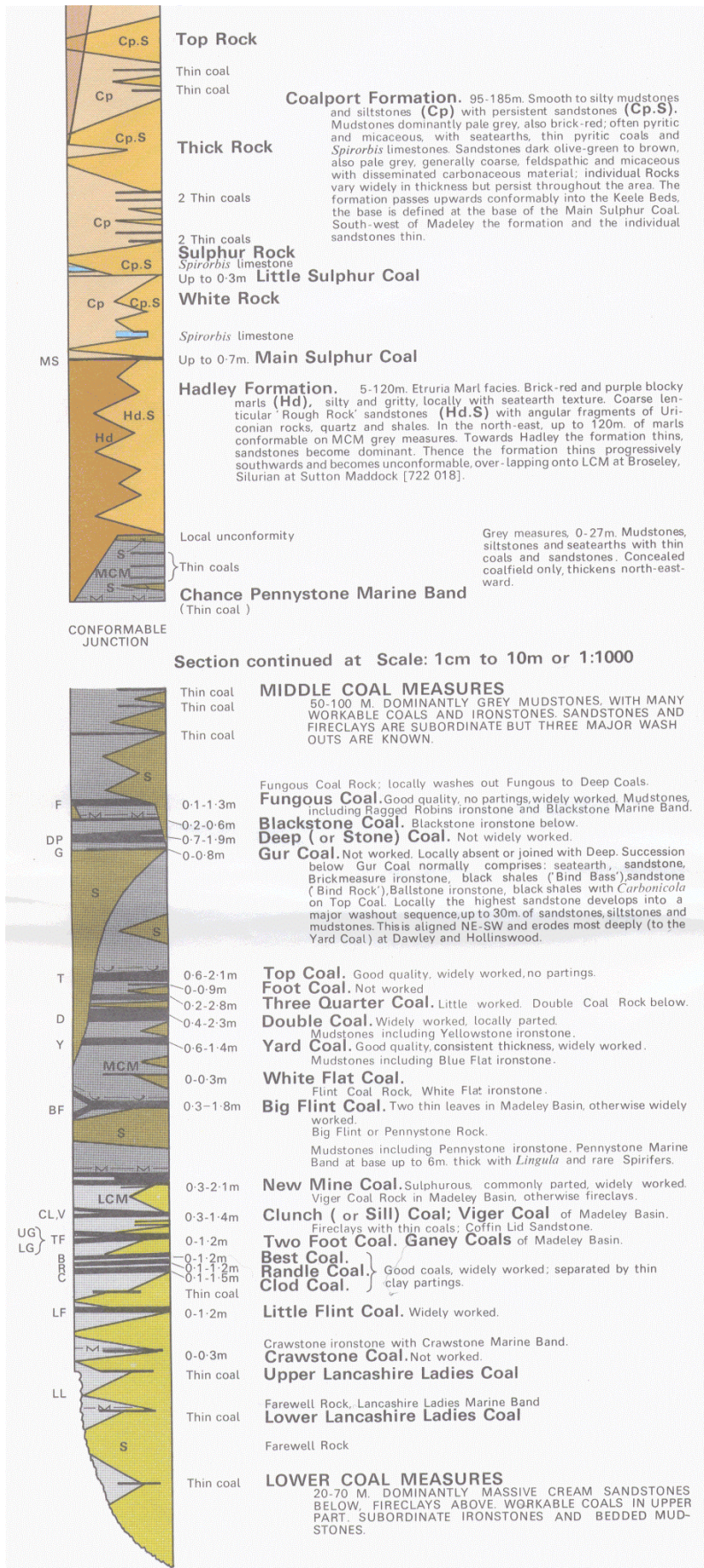
Figure 3 Generalised vertical section of bedrock geology
