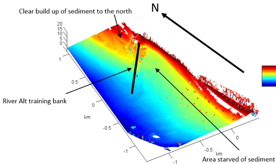
Figure 12: Intertidal elevation analysis December 2016 at Crosby, UK (Image provided by Marlan Maritime Technologies Ltd)
