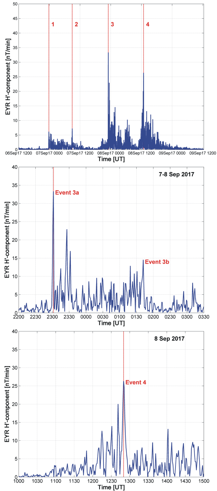
Figure 2. Upper panel: magnitude of the rate of change of the horizontal component ( |H'| ) of the magnetic field observed by the EYR magnetometer during the 6–9 September 2017 series of GMD. Four time periods are marked by red lines, based on the times of four distinct peaks in the magnitude of the rate of change of the H -component of the EYR data, as discussed in the text. Middle panel: detailed examination of the EYR |H'| for the time period around Event 3. Lower panel: as the middle panel, but for the Event 4 time period.
