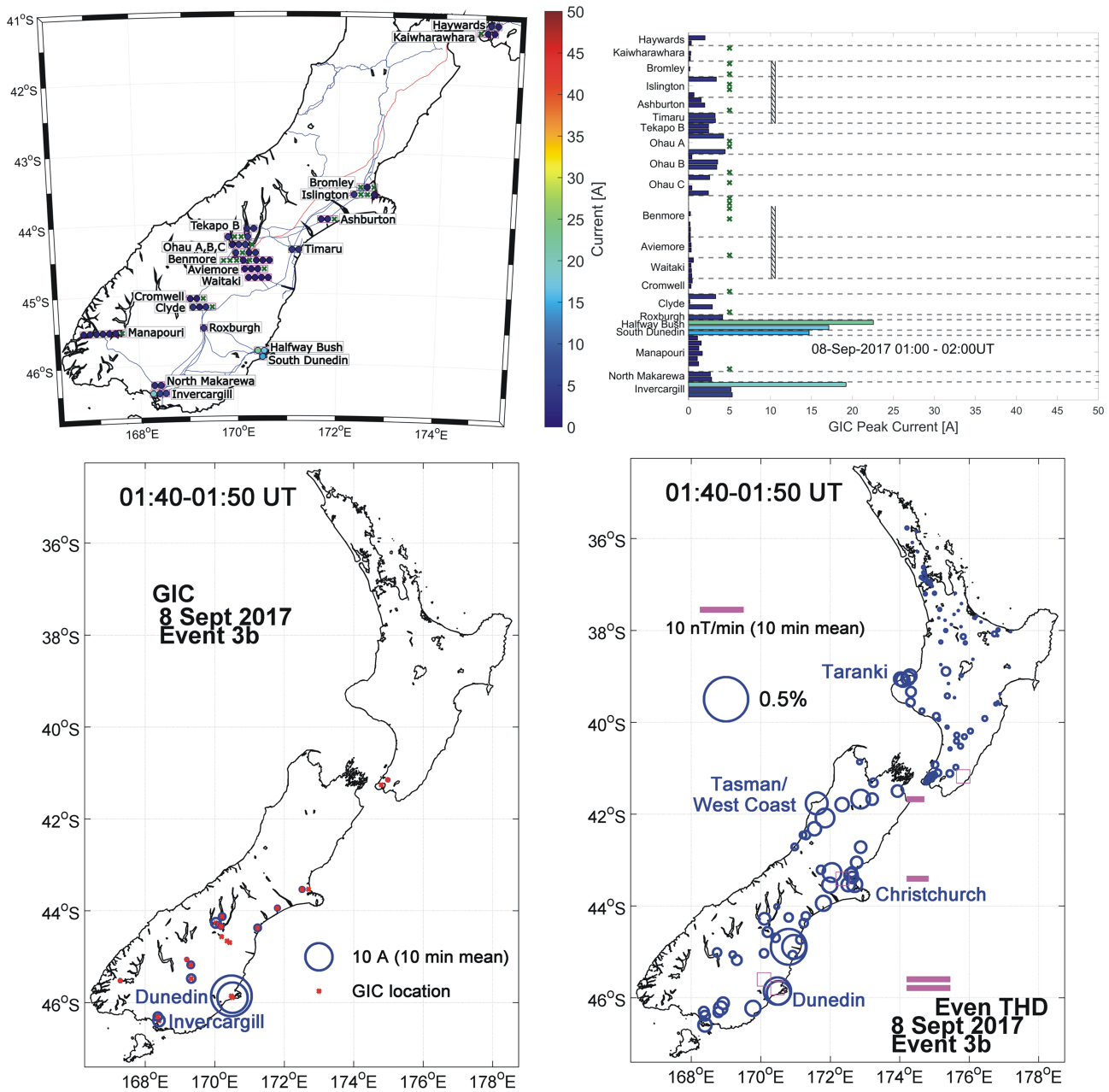
Figure 6. Observations during Event 3b, 2.5 hr after the second sudden commencement solar wind shock arrival. All four panels are in the same format as Figure 5, but for the differing time period, as labeled.
