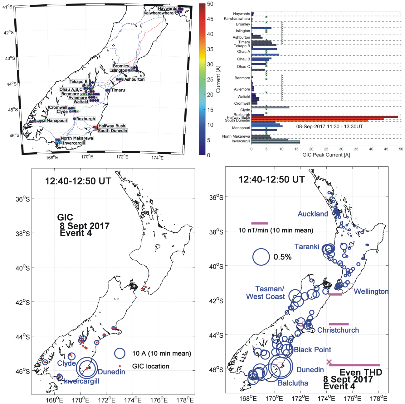
Figure 7. Observations during Event 4, 13.5 hr after the second sudden commencement solar wind shock arrival. All four panels are in the same format as Figure 5, but for the differing time period, as labeled. Note the presence of clear THD increases in the North Island.
