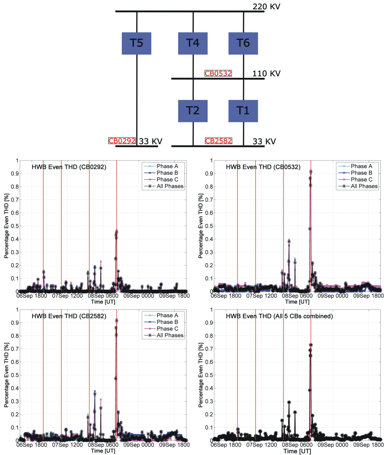
Figure 3. Upper panel: a single line diagram of the Halfway Bush (HWB) substation electrical connections. The red boxes mark HWB T4, and the locations of the five circuit breakers (CB) which have even total harmonic distortion (THD) measurements (see text for more details). Lower panels: even-THD observations at each CB, as labeled, recording separately the three phases and the mean of all phases. The lower right hand panel shows the combined mean of all 15 observations, representing the time-varying summary even-THD for the HWB substation.
