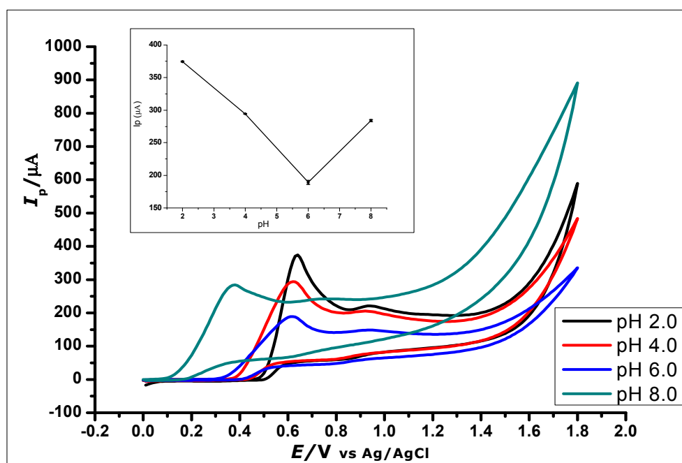
Figure 8. Cyclic Voltammograms showing the effect of pH on the electrochemical behaviour of 1 \times 10^{-2} mol L -1 Gallic Acid at pH range of 2.0–8.0 (Inset). The plot of the Peak Current ( I_p ) against different pH values, showing the effect of pH on the electrochemical behaviour of 1 \times 10^{-2} mol L -1 gallic acid using ZrO 2 nanoparticles modified CPE at a scan rate of 100 mVs -1 .
