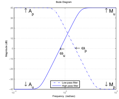
Fig. 4. Weights shape for H_\infty controller design.
