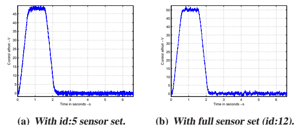
Fig. 12. Limited noise that appears on the control effort with id:5 and id:12.
