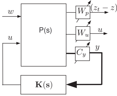
Fig. 3. Multi-objective generalised plant configuration.
