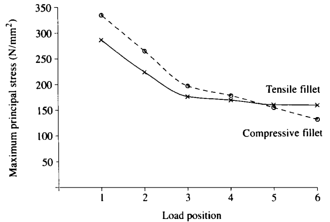
Fig. 7. Fillet stress variation with load position
