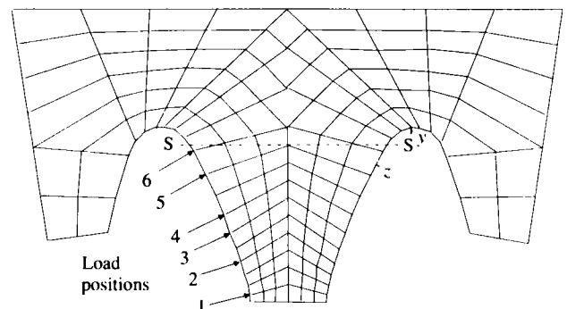
Fig. 12. Finite element mesh of the internal gear
