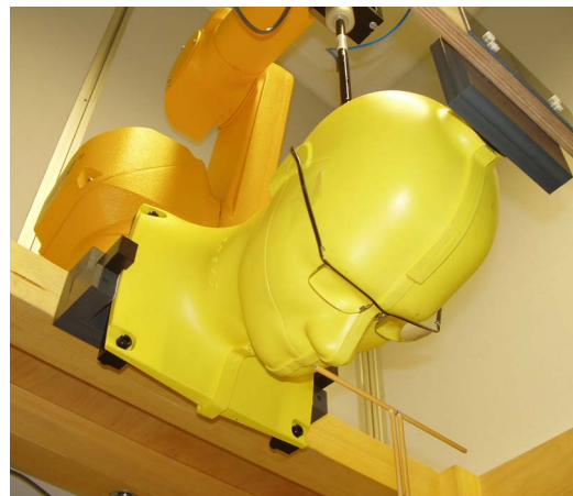
Fig 1 SAR measurement setup showing 900MHz dipole in horizontal alignment and a pair of semi-rimmed spectacles mounted on the SAM head
