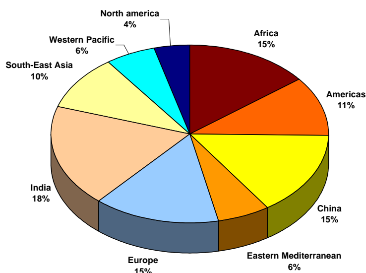
Figure 1: Worldwide road traffic fatalities – 1998 (source WHO 2002)
