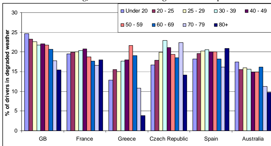
Figure 112: Prevalence of degraded weather conditions amongst passenger car drivers of various ages involved in accidents across Europe and Australia
