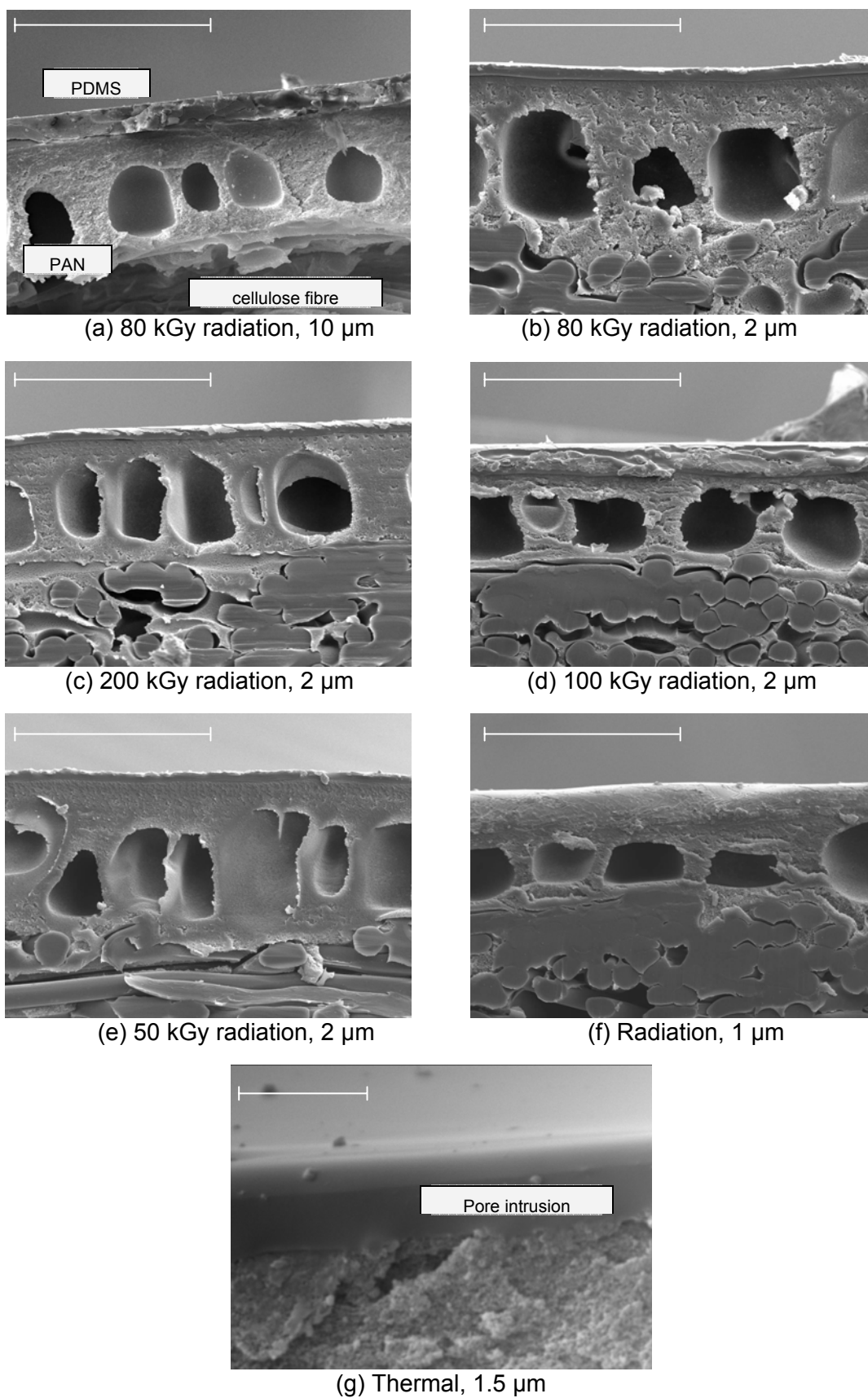
Figure 1: Micrographs of the tested membranes. The dimension on a sub-legend refers to the nominal PDMS thickness in the unswollen state. The size bar represents a length of 60 \mu\text{m} on (a)-(f) and 2 \mu\text{m} on (g).
