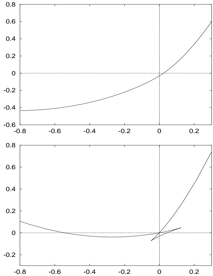
Figure 2: The discriminant surface of the polynomial Q_3 . The critical values of the energy-momentum map are contained in the discriminant surface. The small triangular part for \delta > 0 is not in the image of the energy-momentum map for D < 0 . The figures correspond to the cases of \delta = -0.15 and \delta = 0.15 respectively. ( B = C = -D = \omega = 1.0 )
