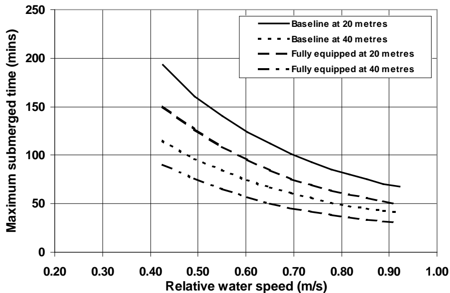
Figure 9 Bottom times for constant depth dives at varying water speeds.
