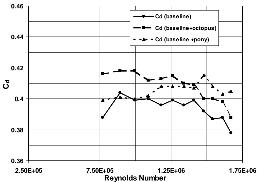
Figure 5 Main configurations against Reynolds number.
