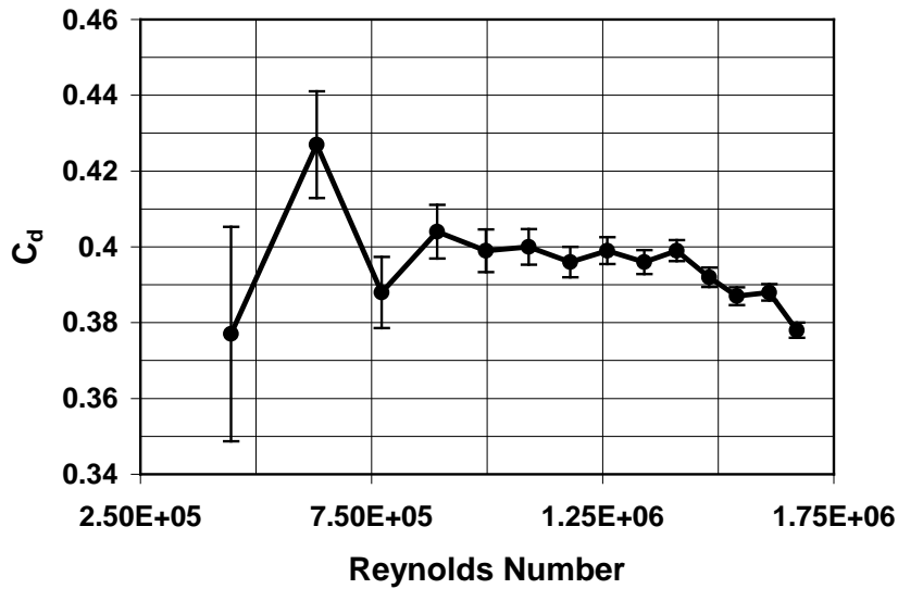
Figure 4 Baseline diver - Reynolds number run.
