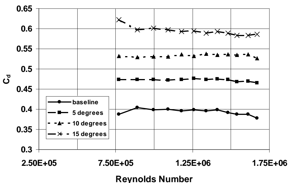
Figure 8 Effect of incidence.
