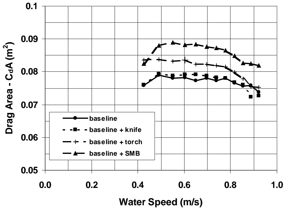
Figure 7 Drag area against water speed for auxiliary equipment.
