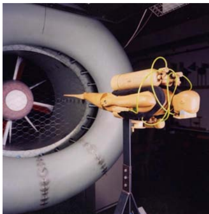
Figure 2 Fully equipped diver - right view
