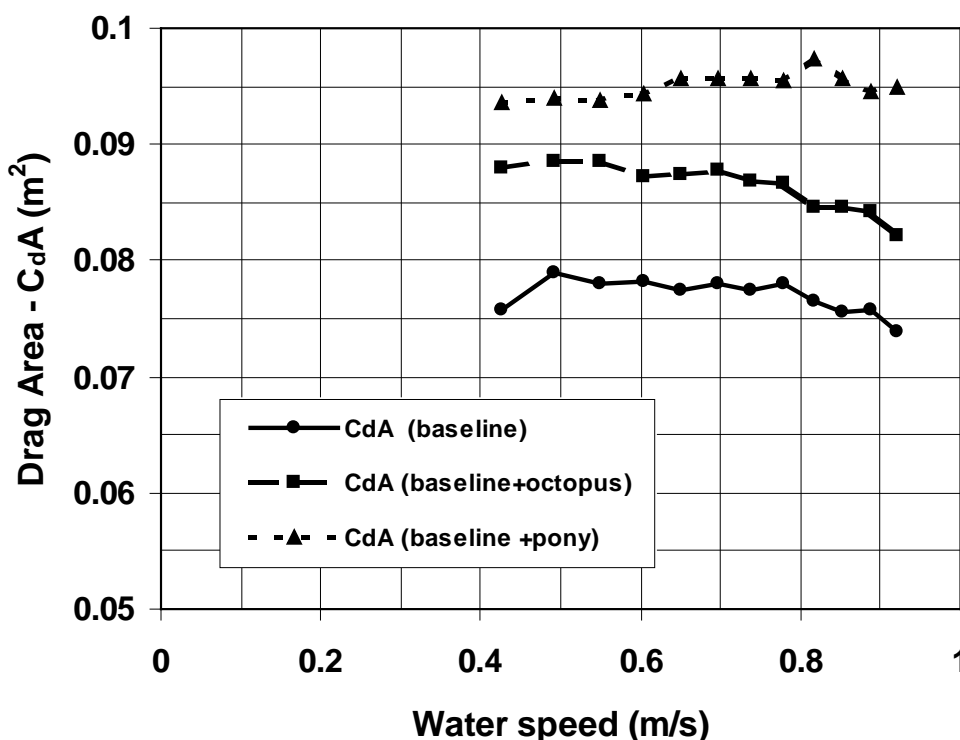
Figure 6 Drag area against water speed for main configurations.
