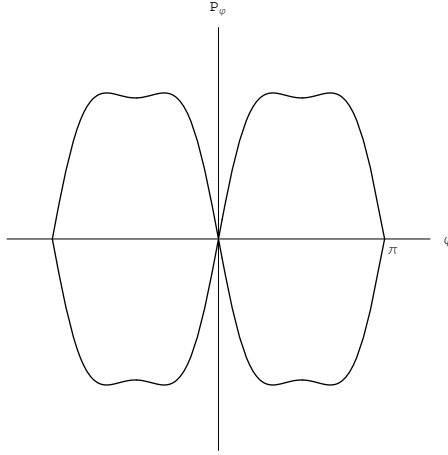
Figure 4: The intersection of the preimage of the isolated singular point (j, g) = (0, 0) with the Poincaré section x_3 = 0 in reduced phase space. The separatrix is of type C_2 before quotient by \mathbb{Z}_2 .
