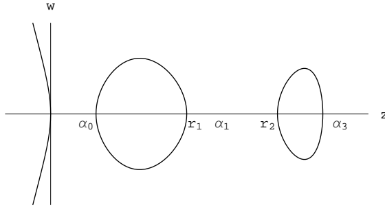
Figure 5: Real part of curve w^2 = -z(z - \alpha_0)(z - r_1)(z - r_2)(z - \alpha_3) showing cycles.
