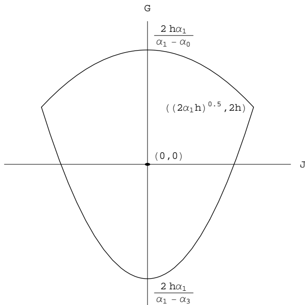
Figure 3: Bifurcation Diagram for the ellipsoid with axis \alpha_0 < \alpha_1 = \alpha_2 < \alpha_3 .
