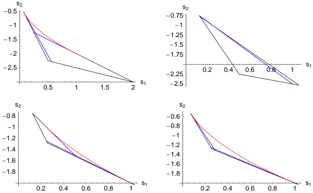
Figure 2: Bifurcation Diagram of almost degenerate Ellipsoids with \alpha_i = (1/4, 1/4 + \varepsilon, 1, 2) , (1/4, 1/2, 1/2 + \varepsilon, 2) , (1/4, 1/2, 1, 1 + \varepsilon) , (1/4, 1/4 + \varepsilon, 1, 1 + \varepsilon) , where \varepsilon = 0.03 .
