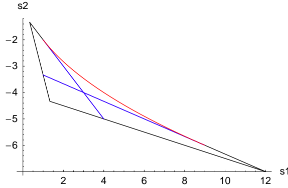
Figure 1: Bifurcation Diagram of the generic Ellipsoid with \alpha_i = 1/3, 1, 3, 4
