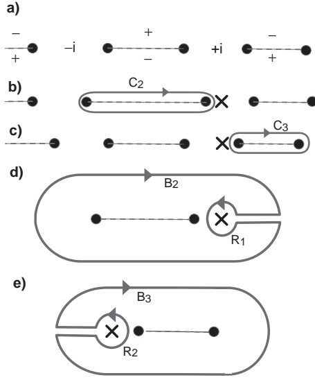
Figure 6: Complex plane \mathbb{C}(s) and choice of branch cuts (a), integration paths for p_\theta for r_1 \rightarrow \alpha_1 (b) and r_2 \rightarrow \alpha_1 (c). (d) and (e) show decomposition of C_2 for case (b) and C_3 for case (c).
