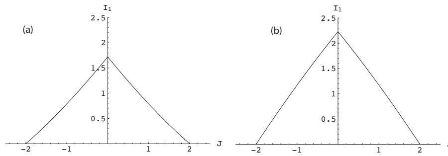
Figure 7: Actions for ellipsoids of revolution: (i) \alpha_0 < \alpha_1 = \alpha_2 , (ii) \alpha_1 = \alpha_2 < \alpha_3 , where \alpha_0 = 1 , \alpha_1 = 2 , \alpha_3 = 4 , h = 1 .
