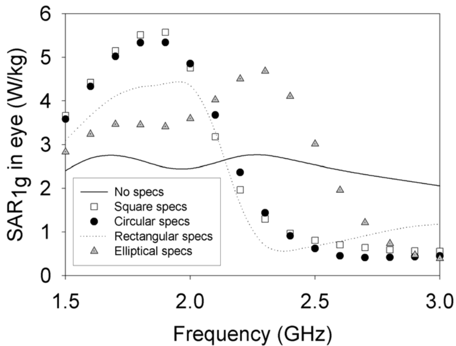
Figure 5. The maximum SAR averaged over 1g in the eye.
