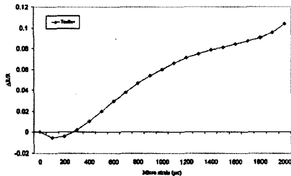
Figure 6. Typical Strain – Resistance plot for Teslin
